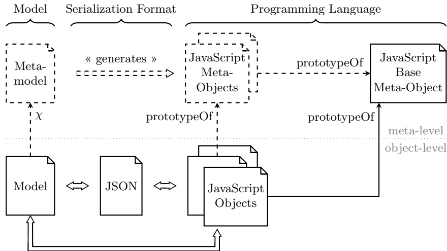
Fig. 1: Architecture of FlexiMeta
