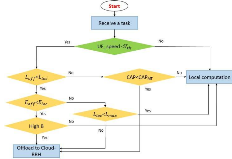
Fig. 3. Proposed offloading decision algorithm for C-RANs
