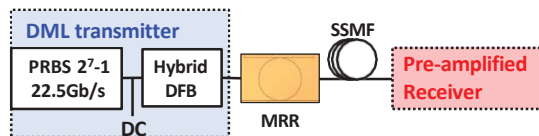
Fig. 4: Experimental setup: DML transmitter, MRR filter for ER and dispersion enhancement, transmission fiber (removed for B2B measurements) and pre-amplified receiver.
