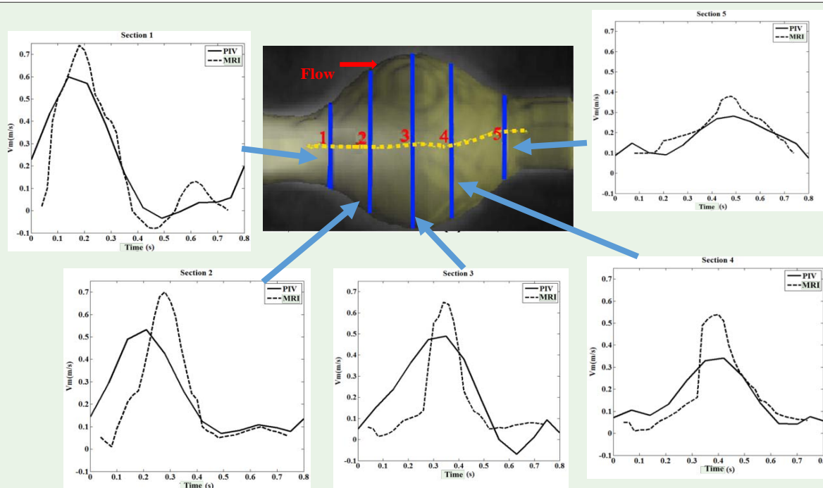
Figure 8: Evolution of the average velocity in cross sections during the cycle determined by MRI and PIV.
