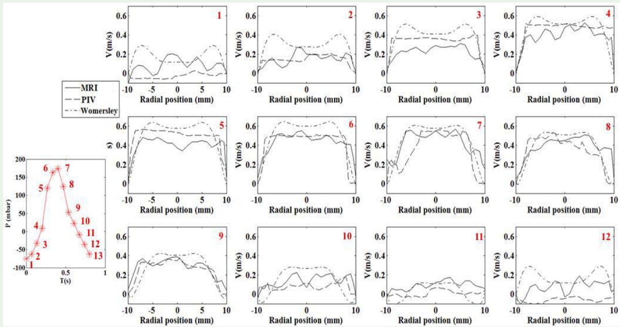
Figure 5: Comparison of experimental results (MRI and PIV measurements) with theoretical results (Wormesley's model) at different pressures of simulated cardiac cycle.
