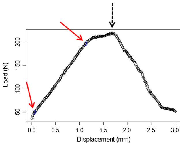
Fig. 4 Load displacement curve selection of two points of the linear part of the curve (red arrow), dot arrow maximal pull-out strength
