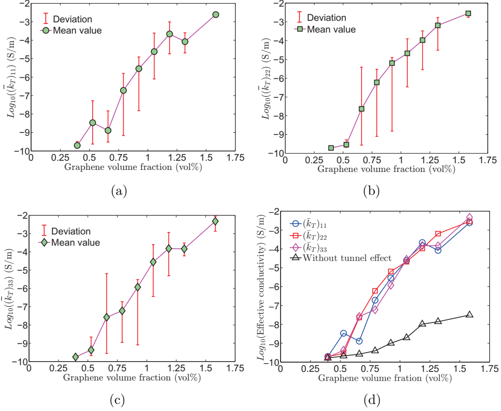
Figure 13: Effective conductivities tensor components as a function of the graphene volume fraction, \bar{E}=1.25 \times 10^{-3} V/nm, \Phi_0 = 0.17 eV. (a) (\bar{k}_T)_{11} (b) (\bar{k}_T)_{22} (c) (\bar{k}_T)_{33} (d) Comparison with the case in which tunnelling effect is neglected.
