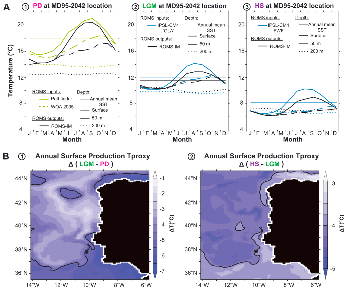
Figure 7. (a) Temperature comparison between forcings (modern climatology IPSL-CM4) and ROMS outputs (mean of the last 10 years of simulation, year 116 to year 125) at MD95-2042 core site, for three climate modes: PD = Present Day (1), LGM = Last Glacial Maximum (2), and HS = Heinrich Stadial (3). (b) Climate mode effect on Tproxy results: LGM-PD (1) and HS-LGM (2) differences for annual surface production Tproxy (mean year 116 to year 125). The black line represents the temperature difference between climate modes recorded at the core site ( \Delta(\text{LGM-PD}) = -5.5^\circ\text{C} and \Delta(\text{HS-LGM}) = -4^\circ\text{C} ).
