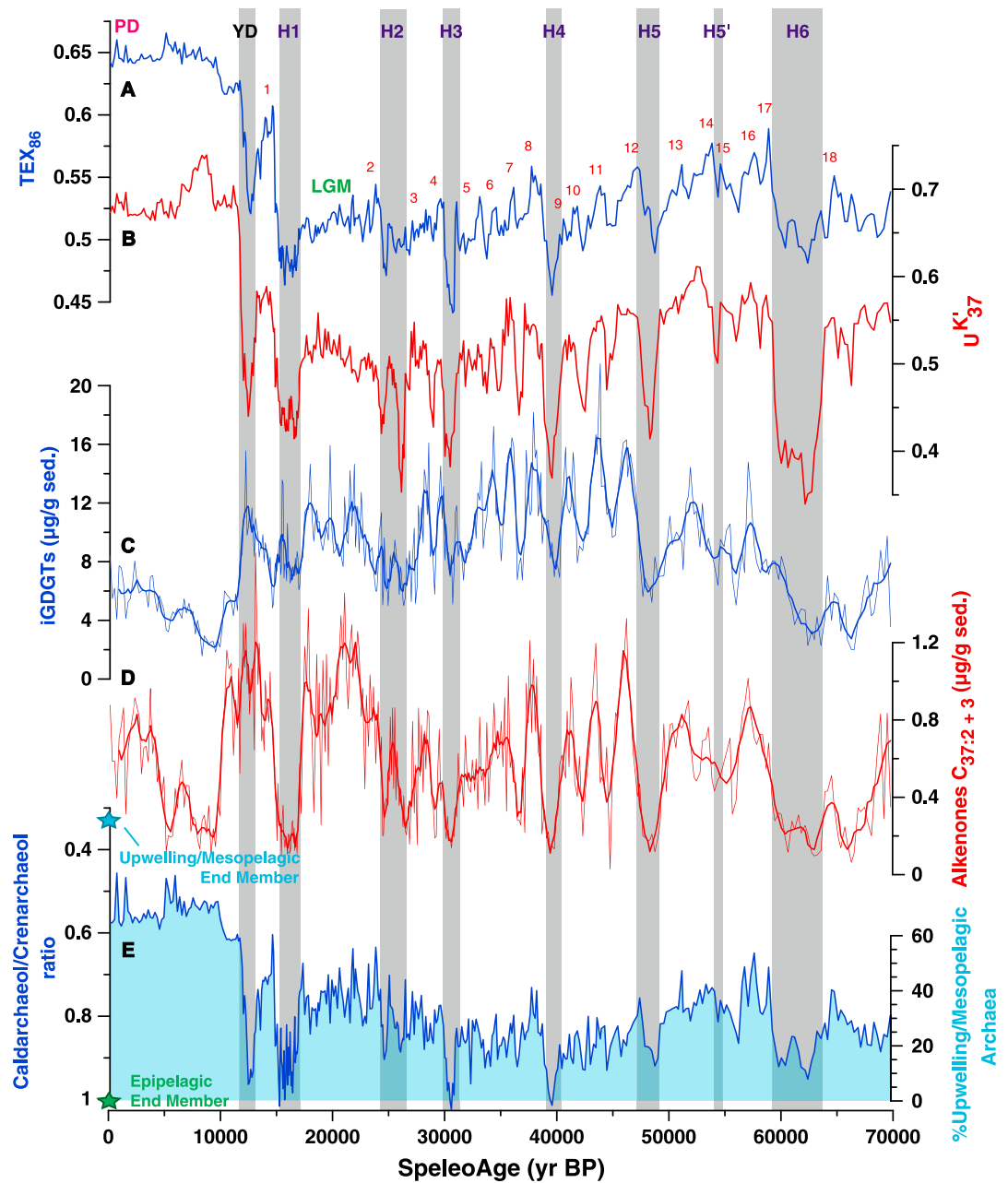
Figure 2. Biomarker results for core MD95-2042. (a) TEX_{86} and (b) U_{37}^{K'} indices and biomarker concentrations (thick line = least squared 2–3 smoothing on 11 points): (c) isoprenoid GDGTs and (d) alkenones C_{37:2} + C_{37:3} . (e) Caldarchaeol/Crenarchaeol ratio (on the left-hand side axis) or contribution of upwelling/mesopelagic Archaea to TEX_{86} signal (on the right-hand axis) calculated after using a bipolar mix model between two Caldarchaeol/Crenarchaeol ratio end-members: light blue and green stars represent “pure” upwelling/mesopelagic Archaea and Epipelagic Archaea end-members, respectively, as proposed by Turich et al. [2007]. Grey bars refer to cold events: YD = Younger Dryas and H1 = Heinrich Stadial 1. Red numbers refer to warm Dansgaard/Oeschger events, also called Greenland Interstadial (GIS) events. PD = Present Day and LGM = Last Glacial Maximum.
