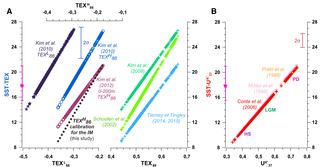
Figure 4. SST reconstructions for core MD95-2042 based on different published linear calibrations. (a) SST-TEX 86 versus TEX index: dark purple stars for TEX 86 L annual mean SST calibration [Kim et al., 2010]; dark blue circles for TEX 86 H annual mean SST calibration [Kim et al., 2010] and associated dark blue 2σ error bar, purple circles for TEX 86 H 0–200 m annual mean SST calibration [Kim et al., 2012], and black dotted line for TEX 86 H annual mean SST calibration for the Iberian Margin (this study); and green crosses [Kim et al., 2008], light green crosses [Schouten et al., 2002], and light blue crosses [Tierney and Tingley, 2014, 2015] for TEX 86 annual mean SST calibrations. (b) SST-U 37 K versus U 37 K : orange crosses for U 37 K culture calibration [Prahl et al., 1988] and pink crosses [Müller et al., 1998] and red crosses with associated red 2σ error bar [Conte et al., 2006] for sedimentary U 37 K annual mean SST calibration. The pink stars represent the present-day annual mean SST at the core site, while the associated pink bars show the maximum and minimum monthly SST at the core site. PD = Present Day; LGM = Last Glacial Maximum; and HS = Heinrich Stadial.
