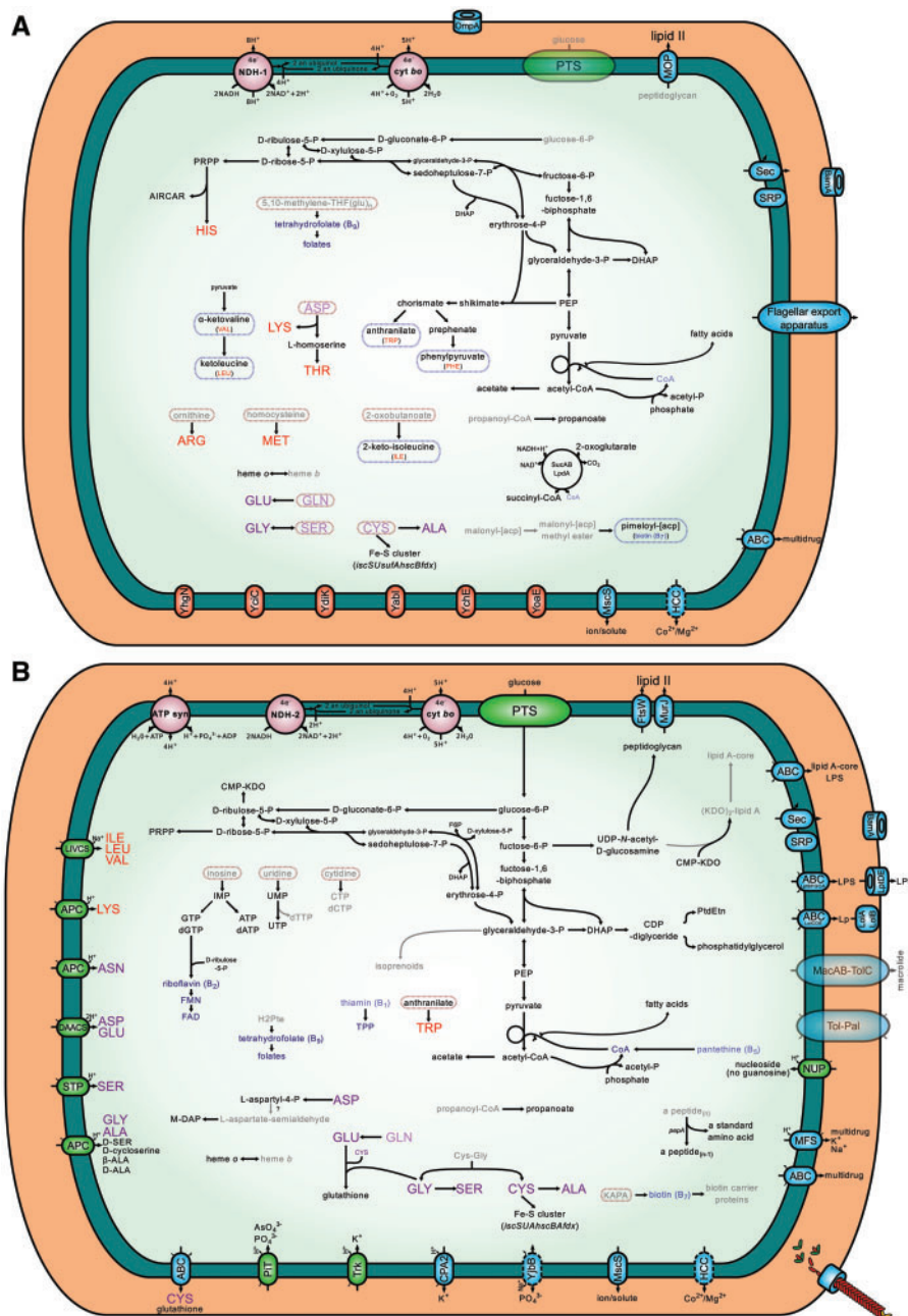
Fig. 4. —Metabolic reconstruction of TuberoLachnus Salignus 's endosymbiotic consortium. Metabolic reconstruction of (A) Buchnera and (B) Serratia symbiotica of T. salignus . Intact pathways are represented with solid black lines, and unclear ones (missing a specific gene or having it pseudogenized by a frameshift) with solid gray lines. Importers are displayed using green ovals, while exporters and exporters/importers are displayed using blue ovals. The name inside each oval states the family/superfamily they belong to (following TCDB's classification [Saier et al. 2014]), otherwise the protein name is used. Essential and nonessential amino acids are shown in red and purple lettering, respectively, while cofactors and vitamins are shown in blue. Blurred compounds represent those for which biosynthesis or import cannot be accounted for based on genomic data. Blurred transporters represent those for which a part of the transporter is missing, therefore recently pseudogenized.
