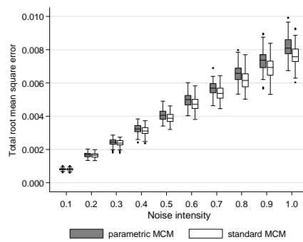
Fig. 3. Quality of the adjustment for the parametric vs. the standard MCM
