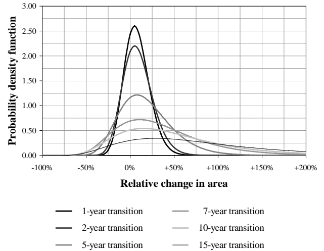
Fig. 2 Evolution of the estimated probability density function of a relative change in area for France
