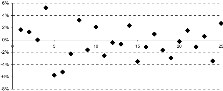
Figure 1- Productivity shocks
