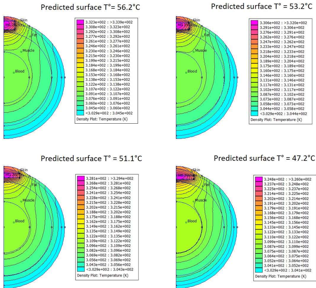
Figure 5. Numerical modeling (FEMM grid with ~7800 nodes) of temperature spatial distribution in and around a subcutaneous pseudotumor placed in the fat layer (3 mm thick) below skin (1 mm) and above muscles for different tumor shapes at constant 100 \mu\text{L} volume. Blood volume is 2.1 mL. MTNs are supposed to dissipate a heat power density p = 2 \text{ W/cm}^3 under an alternating magnetic field of B = 12.8 \text{ mT} at 755 kHz ( H = 10.2 \text{ kA/m} ). Thermal parameters (heat capacity and conductivity) used are taken from literature [22]: ( C_p = 3.28 \text{ J/cm}^3/\text{K} ; k = 0.37 \text{ W/m/K} ) for skin, ( C_p = 1.93 \text{ J/cm}^3/\text{K} ; k = 0.16 \text{ W/m/K} ) for fat, ( C_p = 3.87 \text{ J/cm}^3/\text{K} ; k = 0.48 \text{ W/m/K} ) for muscle, ( C_p = 4.18 \text{ J/cm}^3/\text{K} ; k = 0.6 \text{ W/m/K} ) for blood pool, supposed isothermal at T_0 = 310 \text{ K} . Predicted temperatures at the pseudotumor surface were 56.2, 53.2, 51.1, and 47.2 °C according to pseudotumor cylindrical shape heights of 2.6, 2, 1.34, and 1.04 mm, respectively (for the same 100 \mu\text{L} volume).
