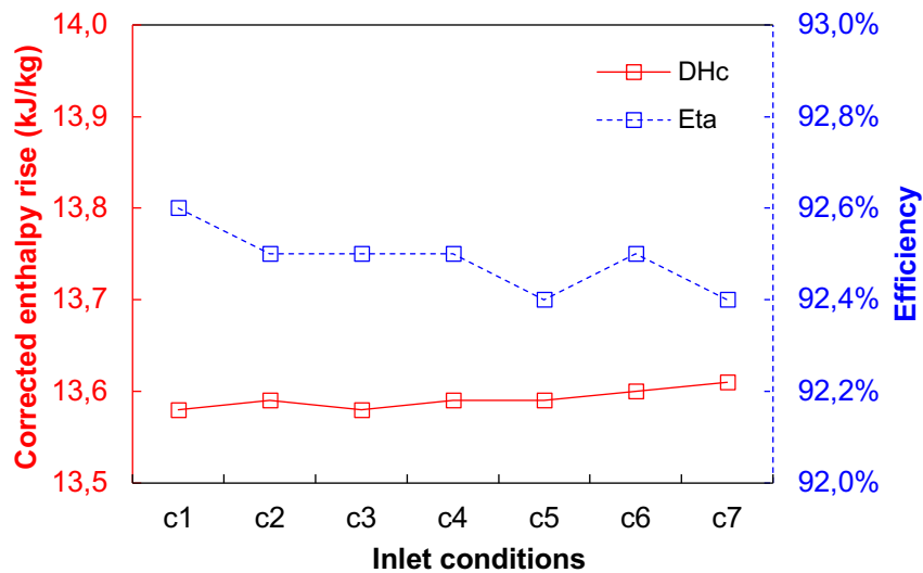
Fig 3: Corrected enthalpy rise (DHc) and efficiency (Eta) at the reference conditions of 27 °C and 8.40 MPa.
