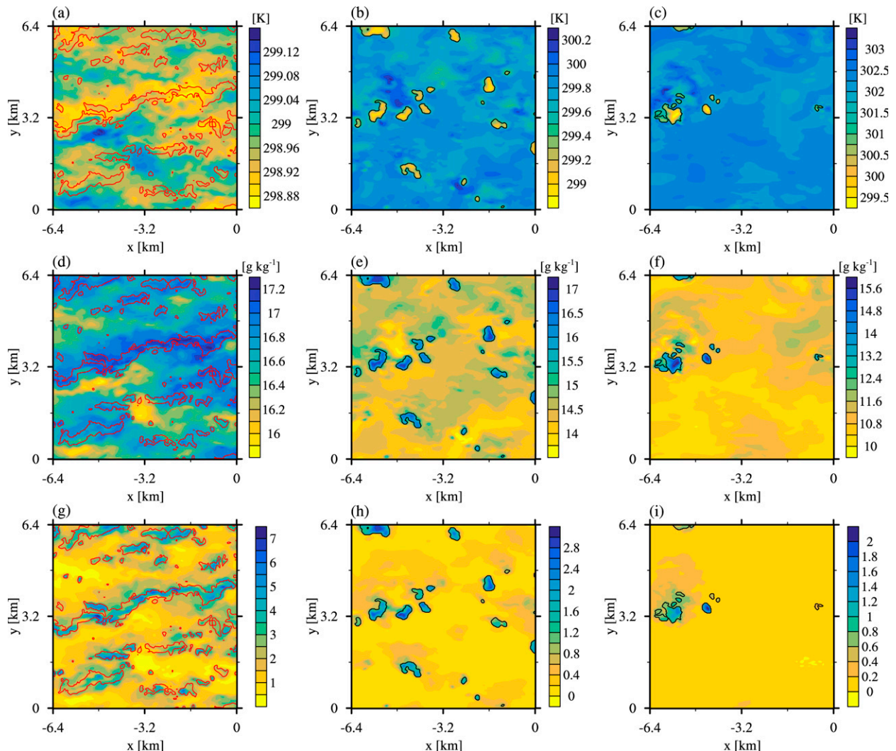
FIG. 5. Fields of coherent liquid water potential temperature at t = 21\,600 s and at z = (a) 350, (b) 850, and (c) 1450 m. (d)–(f) Fields of coherent total water mixing ratio and (g)–(i) fields of the coherent decaying scalar. The black contours of 0.01\text{ g kg}^{-1} liquid water mixing ratio and red contours of 0.4\text{ m s}^{-1} vertical velocity are added. The northwestern quarter of the horizontal domain is shown for clarity.
