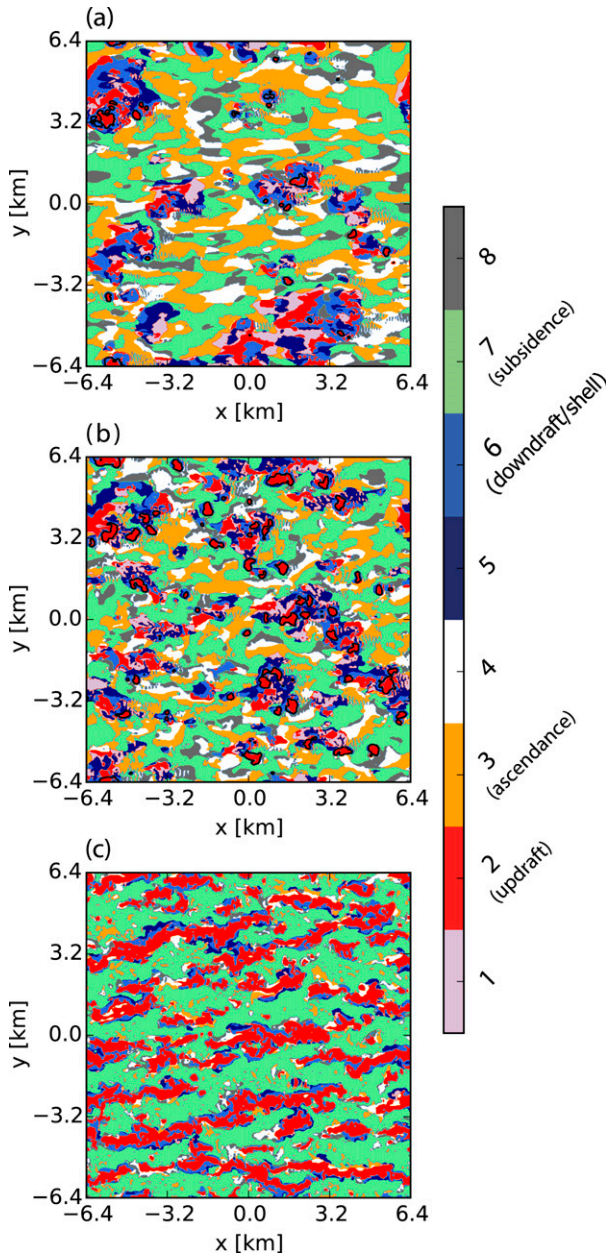
FIG. 8. Fields of octants at t = 21\,600 s and at z = (a) 1450, (b) 850, and (c) 350 m. The contours of 0.01\text{ g kg}^{-1} liquid water mixing ratio are added in (a) and (b).
