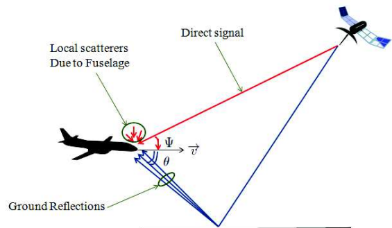
Fig. 1: Illustration of the geometry of the aeronautical communication channel.
