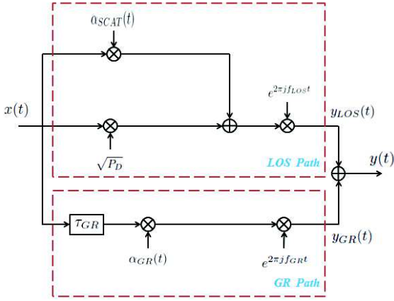
Fig. 3: Aeronautical channel model
