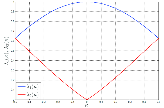
Fig. 4: \lambda_1(\kappa) and \lambda_2(\kappa) as a function of \kappa
