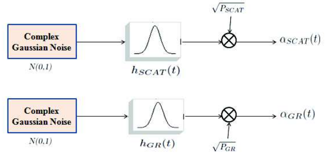
Fig. 2: Blocks generating \alpha_{SCAT} and \alpha_{GR}
