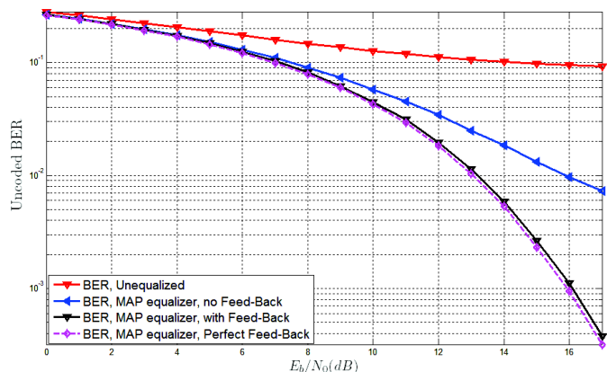
Fig. 9: Uncoded BER 8-PSK, C/M = 6 dB
