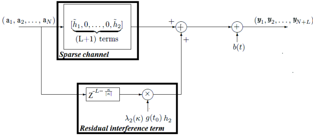
Fig. 6: Discrete equivalent channel model with one term for residual interference
