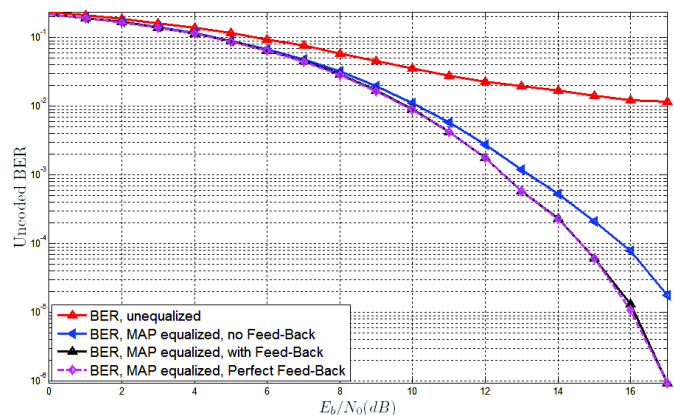
Fig. 8: Uncoded BER BPSK, C/M = 6 dB
