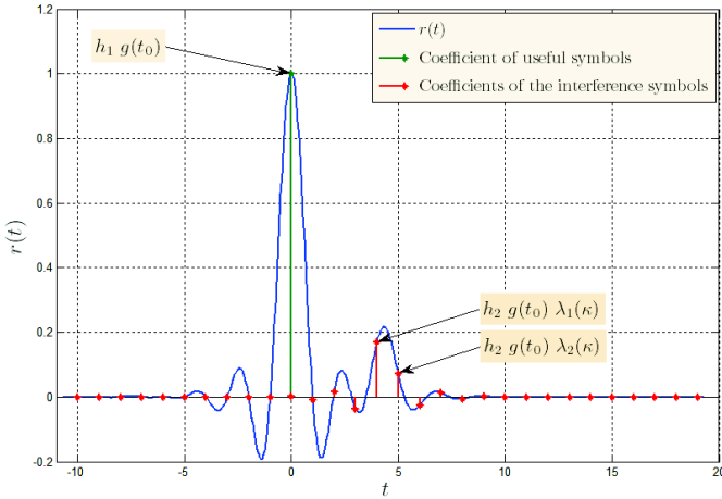
Fig. 5: Discrete equivalent channel filter, t_0 = 0 , \kappa = 0.3 .
