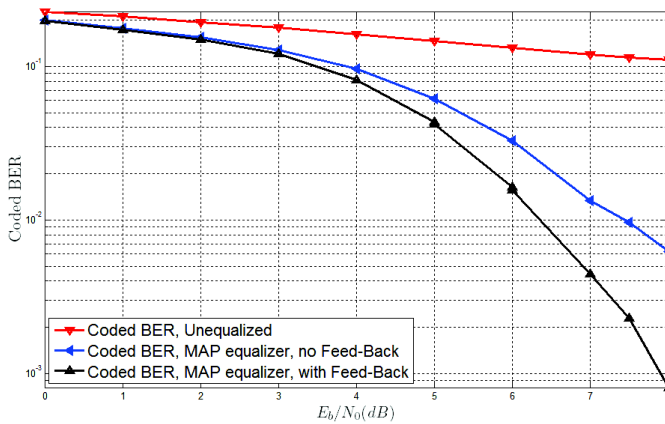
Fig. 11: Coded 8-PSK, C/M = 6 dB
