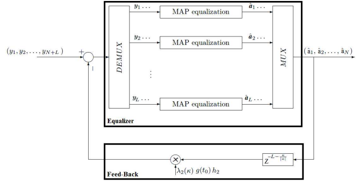
Fig. 7: Proposed MAP equalizer structure
