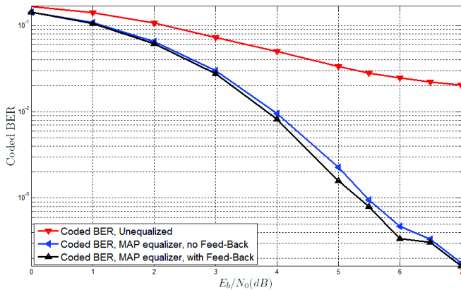
Fig. 10: Coded BPSK, C/M = 6 dB
