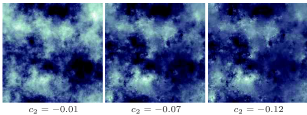
Fig. 1. Realizations of 2D MRW with different values for c_2 .
