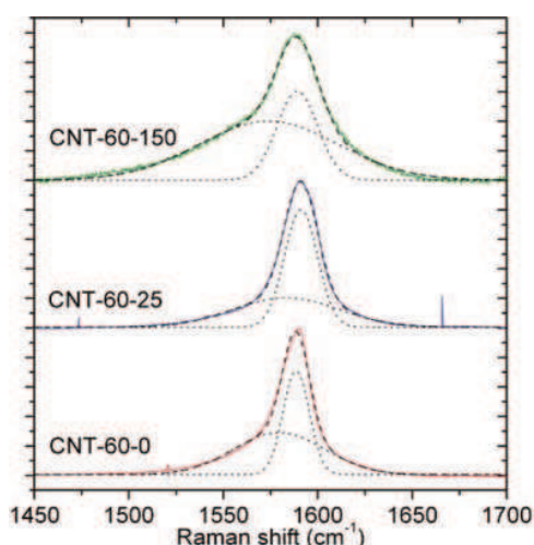
Figure 9. Raman spectra of the G band (ca. 1590 \text{cm}^{-1} ) of CNT-60 samples. The gels have been left unpolarized (CNT-60-0), polarized by applying a sinusoidal 25 mV (CNT-60-25), and 150 mV (CNT-60-150) tension. Each peak is fitted as the sum (dash) of two Gaussian peaks (dot).
