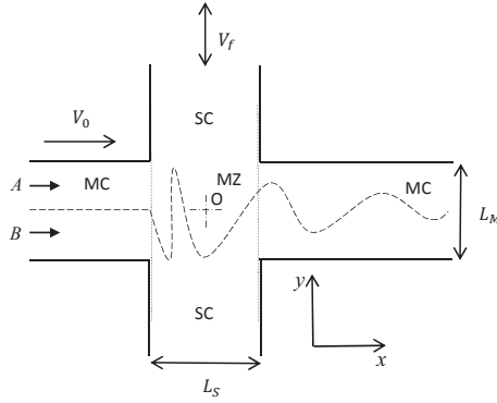
Figure 1: Sketch of the cross-channel micromixer; MC: main channel; SC side channel; MZ: mixing zone; the vertical dotted lines show the investigated region.
