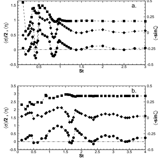
Figure 5: Mean rate of strain, \langle\sigma\rangle , statistical alignment given by \langle-\sin\zeta\rangle and mean growth rate, \langle\eta\rangle , vs. Strouhal number; a. \alpha = 1 ; b. \alpha = 3 ; squares: \langle\sigma\rangle/2 ; diamonds: \langle-\sin\zeta\rangle ; circles: \langle\eta\rangle ; the dashdot line shows the zero value of \langle\eta\rangle .
