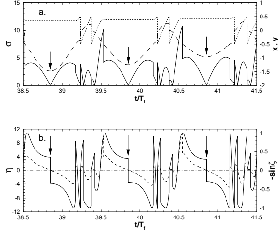
Figure 7: Lagrangian signals for \alpha = 1 and St = 0.125 ; a. solid line: \sigma ; short dash: x ; long dash: y ; b. solid line: -\sin \zeta ; dashed line: \eta ; each arrow shows a turning back in a side channel.
