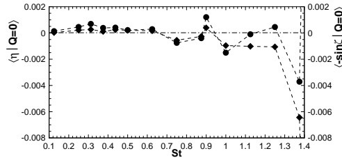
Figure 9: Mean values of -\sin \zeta and \eta conditioned on pure shear vs. Strouhal number; \alpha = 3 ; diamonds: \langle -\sin \zeta | Q = 0 \rangle ; circles: \langle \eta | Q = 0 \rangle .
