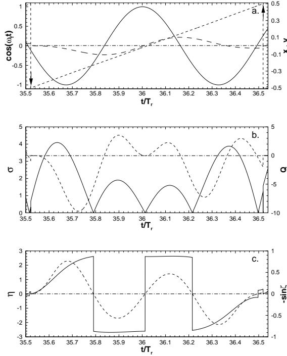
Figure 12: Lagrangian signals for \alpha = 1 and St = 1.5 ; a. solid line: \cos \omega_f t ; short dash: x ; long dash: y ; the arrows show the injection and exit of the Lagrangian particle; b. solid line: \sigma ; dashed line: Q ; the dashdot line shows the zero value of Q ; c. solid line: -\sin \zeta ; dashed line: \eta .
