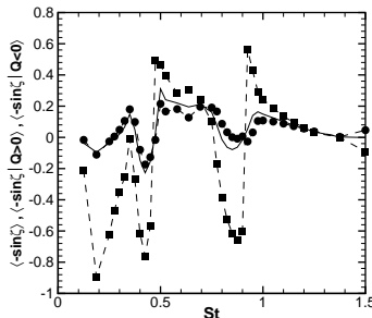
Figure 13: Statistical orientation of tracer gradient; \alpha = 1 ; solid line: \langle -\sin \zeta \rangle ; squares: conditioning on hyperbolic events, \langle -\sin \zeta | Q > 0 \rangle ; circles: conditioning on elliptic events, \langle -\sin \zeta | Q < 0 \rangle .
