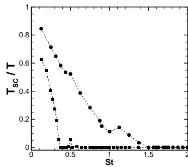
Figure 6: Mean ratio, T_{sc}/T , of time spent in the side channels during a simulation; squares: \alpha = 1 ; circles: \alpha = 3 .
