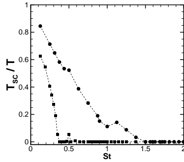
Figure 6: Mean ratio, T_{sc}/T , of time spent in the side channels during a simulation; squares: \alpha = 1 ; circles: \alpha = 3 .
