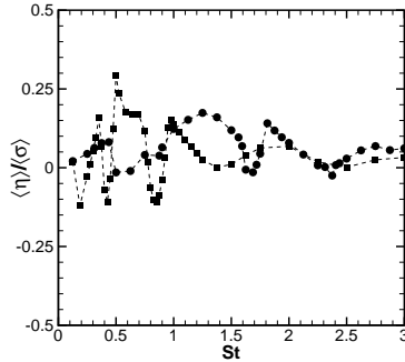
Figure 4: Ratio of mean growth rate to mean rate of strain, \langle \eta \rangle / \langle \sigma \rangle , vs. Strouhal number; squares: \alpha = 1 ; circles: \alpha = 3 .
