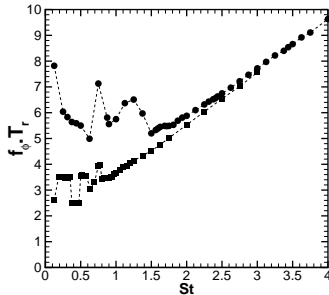
Figure 10: Mean tilting frequency of the strain principal axes normalised by the mean residence time in the mixing cavity vs. Strouhal number; squares: \alpha = 1 ; circles: \alpha = 3 .
