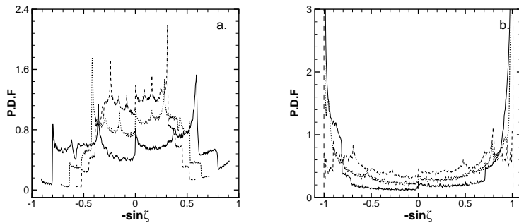
Figure 11: P.d.f's of tracer gradient orientation; a. \alpha = 1 ; b. \alpha = 3 ; solid line: St = 2 ; short dash: St = 3 ; long dash: St = 4 .
