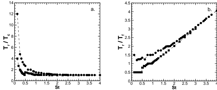
Figure 2: Mean residence time in the micromixer cavity; a. T_r/T_c , with T_c = L_S/V_0 being the convection timescale; b. T_r/T_f , with T_f being the time period of the flow forcing; squares: \alpha = 1 ; circles: \alpha = 3 .
