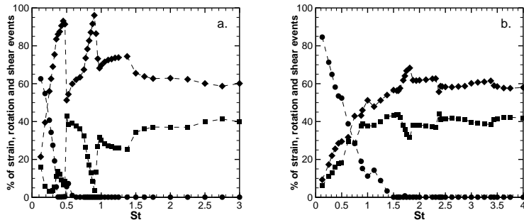
Figure 3: Ratios of strain-, rotation- and shear-dominated events along the Lagrangian paths vs. Strouhal number; a. \alpha = 1 ; b. \alpha = 3 ; squares: strain; diamonds: rotation; circles: shear.
