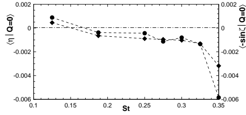
Figure 8: Mean values of -\sin \zeta and \eta conditioned on pure shear vs. Strouhal number; \alpha = 1 ; diamonds: \langle -\sin \zeta | Q = 0 \rangle ; circles: \langle \eta | Q = 0 \rangle .
