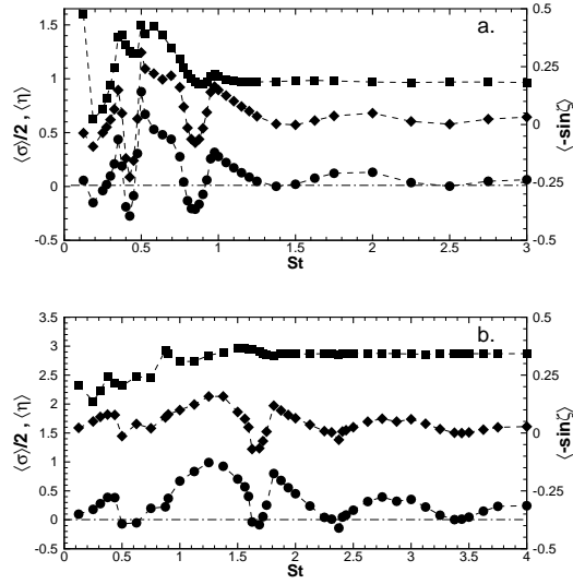
Figure 5: Mean rate of strain, \langle \sigma \rangle , statistical alignment given by \langle -\sin \zeta \rangle and mean growth rate, \langle \eta \rangle , vs. Strouhal number; a. \alpha = 1 ; b. \alpha = 3 ; squares: \langle \sigma \rangle / 2 ; diamonds: \langle -\sin \zeta \rangle ; circles: \langle \eta \rangle ; the dashdot line shows the zero value of \langle \eta \rangle .
