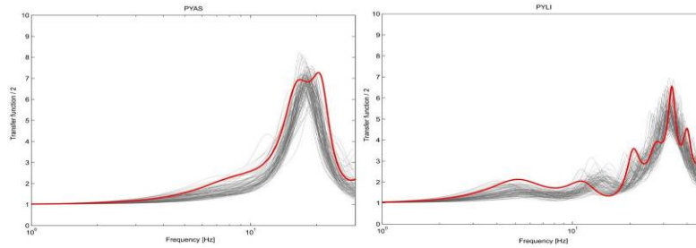
Figure 10 – 1D transfer functions computed with “best estimated” Vs30 profile (red) and the one thousand profile sets deriving from the “acceptable misfit” approach (gray) for both PYAS and PYLI sites.
