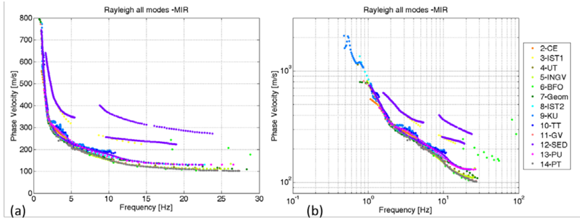
Figure 2 – Mirandola: comparison of the dispersion curves provided by the teams. Only the dispersion curves of all the modes of Rayleigh wave are shown. In a) the dispersion curves are reported in linear scale of frequency and phase velocity while in b) the dispersion curves are reported in a log scale of both frequency and phase velocity.
