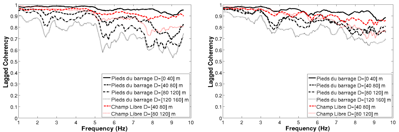
Fig. 5 – Estimated lagged coherency as a function of frequency for the NS (left) and EW (right) component; the median value of all the events within each distance bin along the dam-foundation interface (black lines) and on the free field (red lines).
