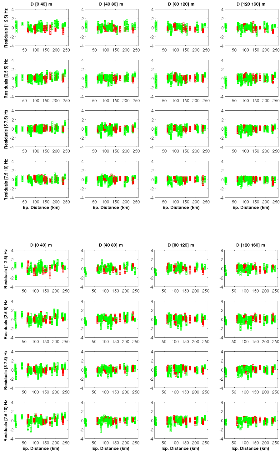
Fig. 7 – Coherency residuals of individual median estimates of ATANH(Lagged) coherency for each event with respect to the global median (ATANH units) of all the events as a function of epicentral distance of the NS (up) and EW (down) component for magnitude bins of M [1,5 2,5] (green) and M [2,5 4,1] (red).
