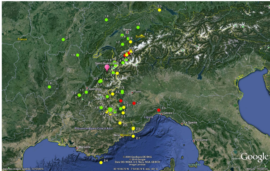
Fig. 3 – Map of the subset of 67 events, recorded from the seismological array during the period of six months (June 2015- December 2015). Green circles represent event locations with M_L [1.5 2), yellow circles M_L [2 3) and red circles M_L [3 4,1]. The pink balloon indicates the location of the arch dam.
