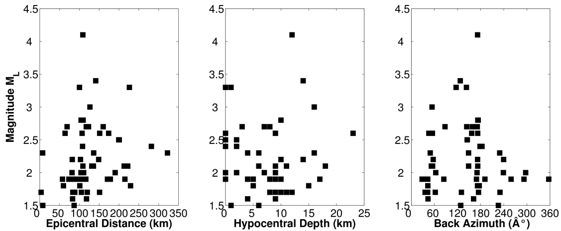
Fig. 4 – Magnitude distribution, M_L , as a function of epicentral distance (km) (left), depth (km) (middle) and Back Azimuth ( ^\circ ) for the subset of 67 events selected for analysis.
