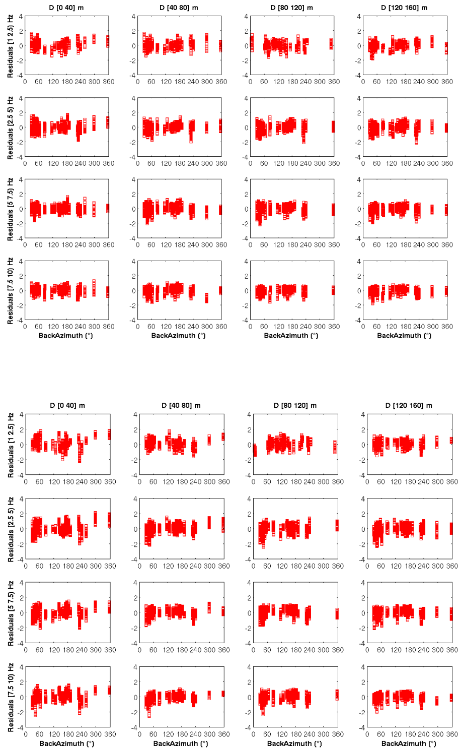
Fig. 8 – Coherency residuals of individual median estimates of ATANH(Lagged) coherency for each event with respect to the global median (ATANH units) of all the events as a function of back azimuth of the NS (up) and EW (down) component.
