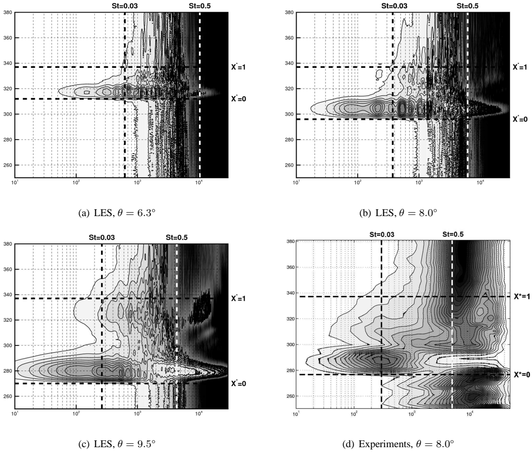
Fig. 5: Frequency–streamwise location map of the magnitude of the wall pressure pre-multiplied spectra normalized by the local value of the variance (arbitrary scale). Abscissa: frequency in Hz, with Strouhal number St_L of values 0.03 and 0.5 indicated. Ordinate: streamwise coordinate, with dimensionless streamwise coordinate X^* values of 0 and 1 indicated.
