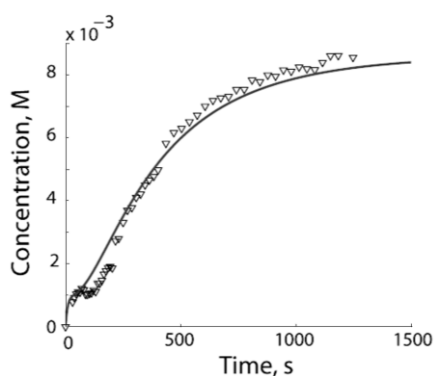
Figure 3. Kinetics of polarized NMR line of alkene a(-H) during thermolysis of 0.02 M solution of 3a (b) in m\text{-C}_6\text{D}_4\text{Cl}_2 at 386 K in the presence of 6 eq of thiophenol: symbols—experimental data points, solid lines—calculated dependence vs. time.
