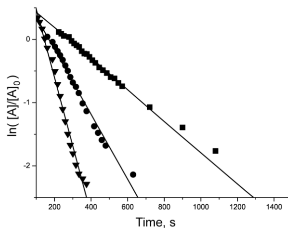
Figure 4. Kinetics of CIDNP on alkoxyamine 1a during thermolysis of 0.02 M solution of alkoxyamine in FSol in the presence of thiophenol and its fit (line) with monoexponent in semi-logarithmic scale: 361 K, [PhSH] = 0.1 M (■), 373 K, [PhSH] = 0.136 M (●), 398 K, [PhSH] = 0.13 M (▼). The values of k_{\text{obs}} obtained from the fit: 361 K— k_{\text{obs}} = 2.0 \times 10^{-3} \text{ s}^{-1} , 373 K— k_{\text{obs}} = 5.0 \times 10^{-3} \text{ s}^{-1} , 398 K— k_{\text{obs}} = 1.5 \times 10^{-2} \text{ s}^{-1} .
