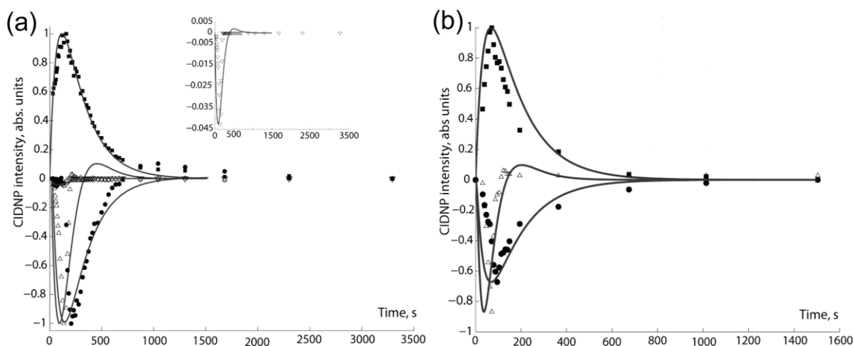
Figure 2. Kinetics of polarized signals (normalized) during thermolysis of 0.02 M solution of alkoxyamines in FSol 2a (a) at 386 K in the presence of 3 eq. of thiophenol and 3a (a) at 386 K in m\text{-C}_6\text{D}_4\text{Cl}_2 in the presence of 6 eq of thiophenol: (■)—alkoxyamine 2a , (●)—alkane aH , (Δ)—dimer aa , (∇)—alkene a(-H) . (b): (■)—alkoxyamine 3a , (●)—alkane aH , (Δ)—dimer aa . Inset—the kinetics of CIDNP on a(-H) for 2a . Inset: enlargement of evolution of CIDNP signal for a(-H) —(∇) of 2a . Solid line—calculated dependence of CIDNP vs. time.
