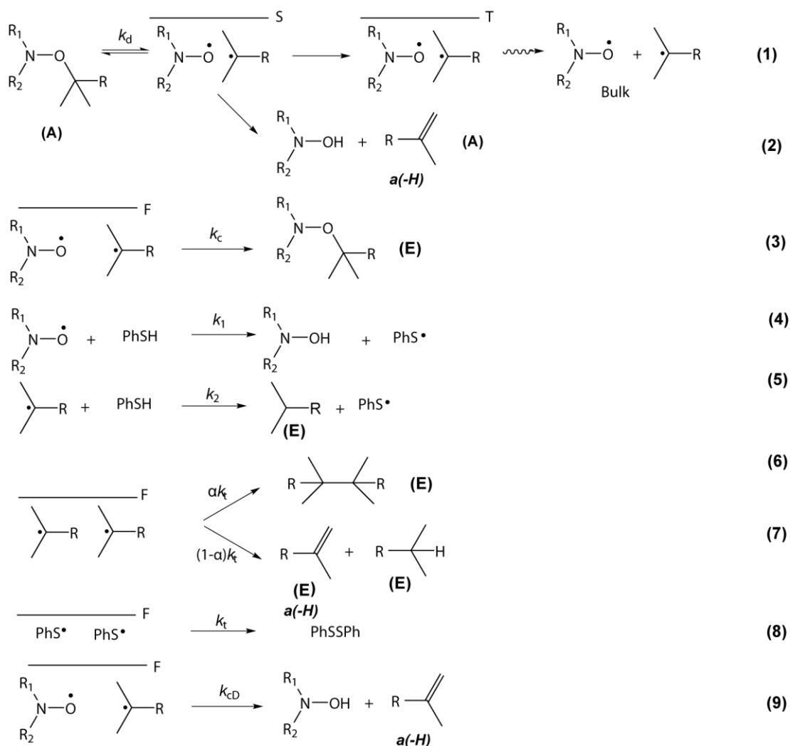
Scheme 2. The kinetic scheme of decomposition of alkoxyamine in the presence of thiophenol. Letters in brackets indicate the sign of CIDNP: A —absorption, E —emission.
