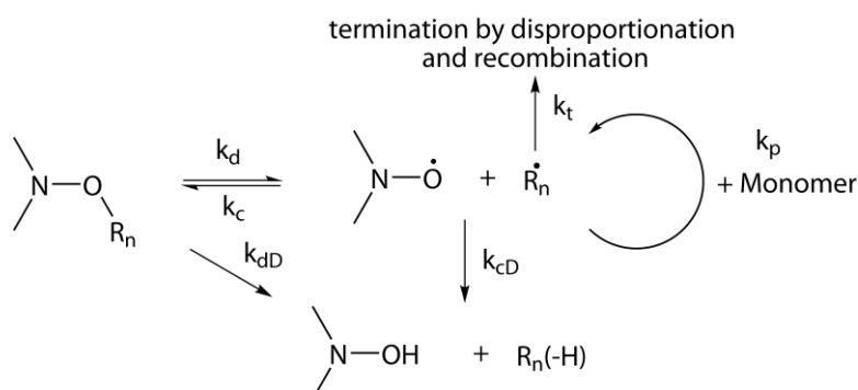
Scheme 1. The mechanism of NMP with side reactions of H-atom transfer.
