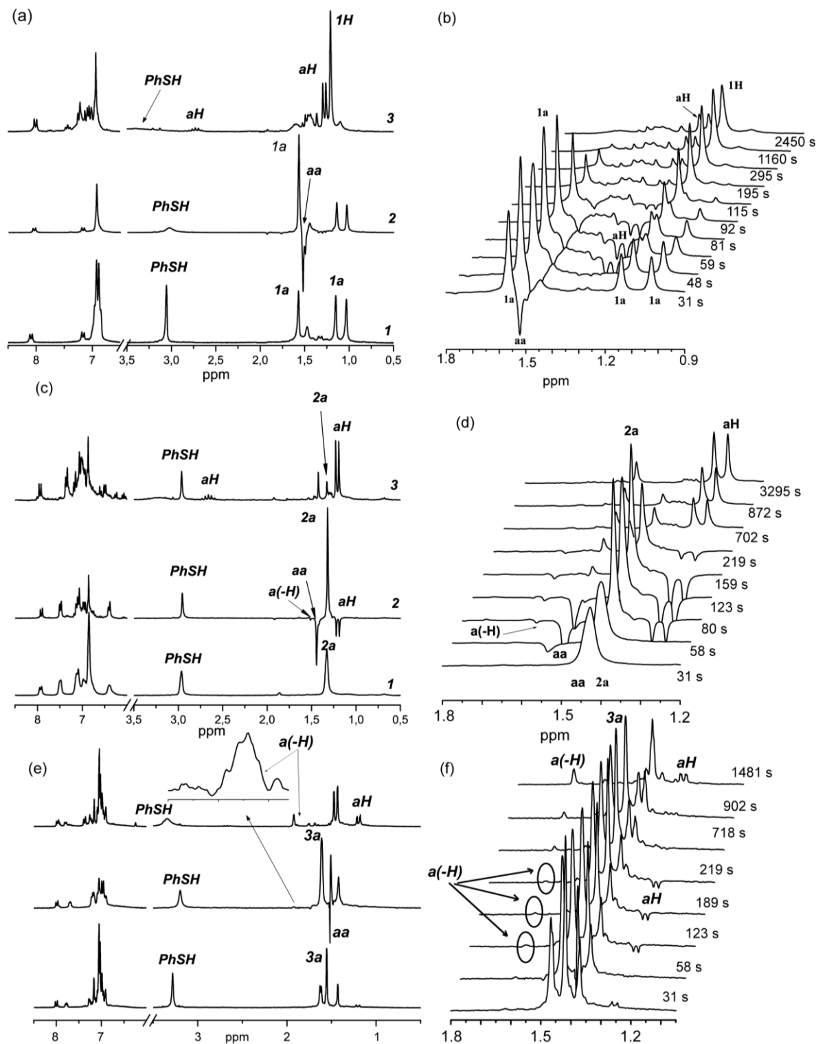
Figure 1. ^1\text{H} NMR spectra recorded at room temperature before (1) and after (3) thermolysis of 1a (a), 2a (c) in FSol and 3a (e) in m\text{-C}_6\text{D}_4\text{Cl}_2 and spectra with polarized signals obtained during the thermolysis (2). ^1\text{H} NMR spectra recorded at different time intervals from the beginning of the reaction during thermolysis of 1a (b) at 398 K, 0.02 M solution of alkoxyamine in FSol, 5.5 eq of thiophenol, 2a (d) at 386 K, 0.02 M solution of alkoxyamine in FSol, 3 eq of thiophenol, 3a (f) at 386 K, 0.02 M solution of alkoxyamine in m\text{-C}_6\text{D}_4\text{Cl}_2 , 6 eq of thiophenol. Signs of polarization: E — aa , a(-H) , aH ; A — 1a – 3a . Inset: enlargement of the chemical shift zone for a(-H) of 3a .
