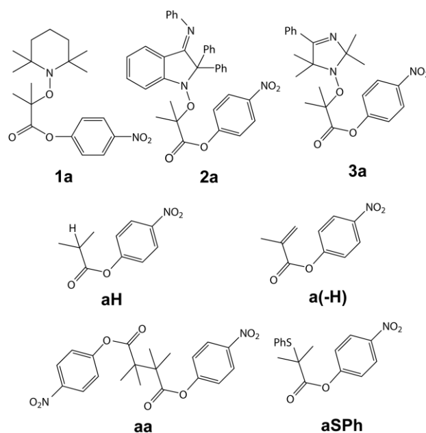
Chart 1. The structures of alkoxyamines and products of decomposition.
