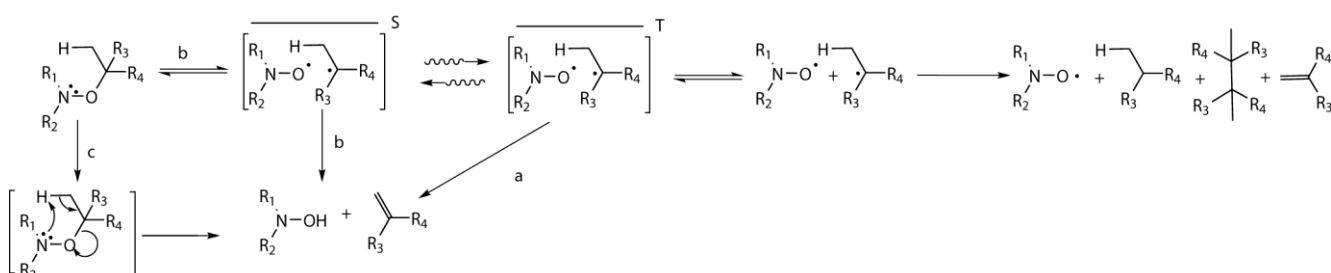
Scheme 3. The different pathways affording the generation of alkene during the decomposition/reformation of alkoxyamine.
