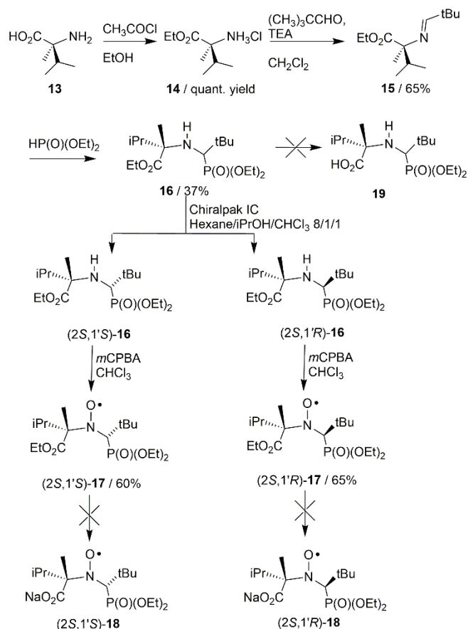
31 Scheme 3. Synthesis of diastereomeric \alpha -aminophosphonates esters 16 and 32 related nitroxides esters 17 .
