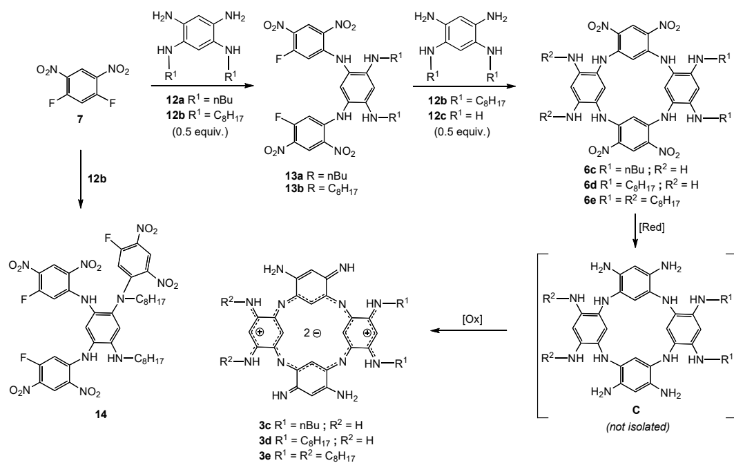
Scheme 3. Synthesis of N-substituted azacalixpyrin 3c-e .
