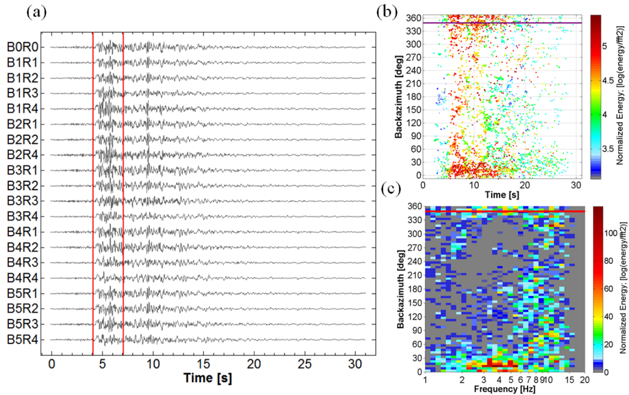
Fig. 3 – (a) EW component velocity time series recorded at the array stations for the event occurred on February 02, 2014 at 01:23:13 UTC ( M_L = 3.5 , Baz= N 348°, R_{epi} = 13 km, H=31 km). Entire signal length has been used for wavefield analysis and the segment between the red lines for coherency analysis. (b) Backazimuth distribution of the wavefield of the same event as a function of time. (c) 2D Histogram of the backazimuth as a function of frequency. Red line indicates the backazimuth of the event and colorbar the normalized energy.
