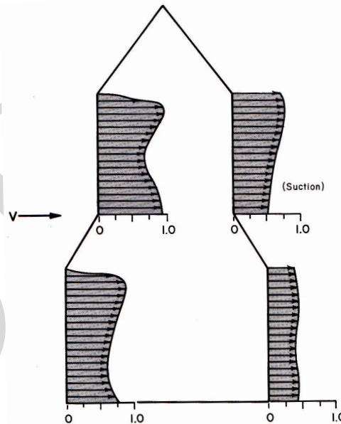
Figure 10: Distribution of C_D on a Gothic-Gathedral, according to [?].
