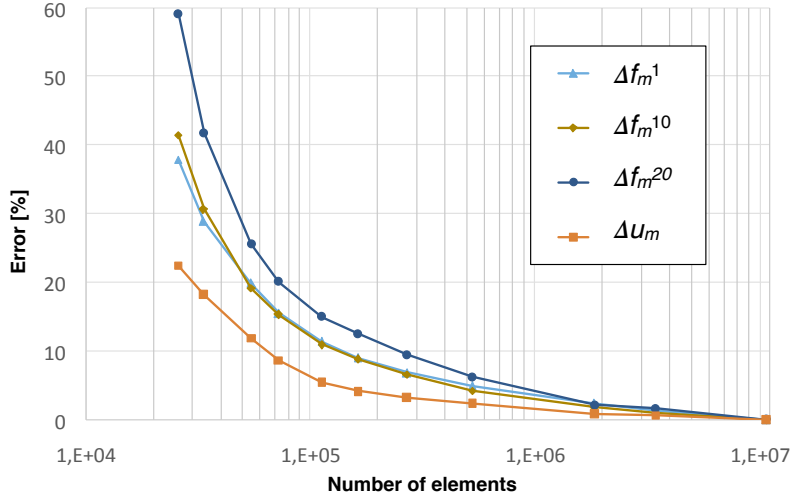
Figure 20: Relative error for three eigenfrequencies and the vertical displacement of point V as function of the elements number of each mesh m .
