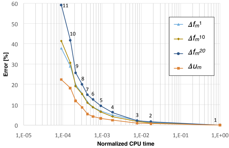
Figure 22: Normalized CPU times versus relative errors for three eigenfrequencies and the vertical displacement of point V; numbers 1 to 11 indicate the mesh m .
