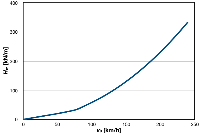
Figure 16: Total horizontal wind thrust H_w versus v_0 .
