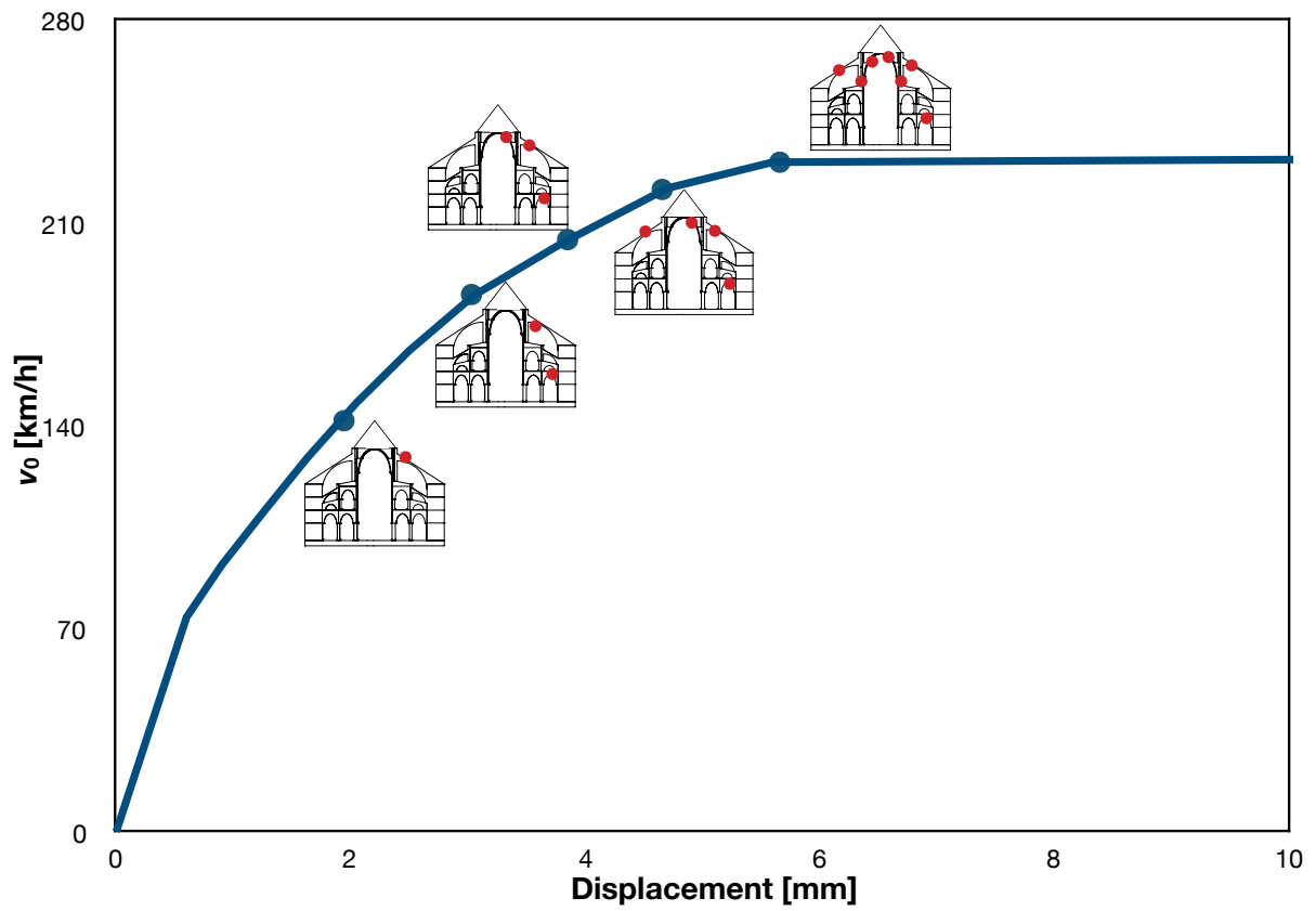
Figure 18: The failure sequence of the Cathedral; the dots on the Cathedral sections indicate the formation of a severe damage, leading to a plastic hinge or a sliding zone.
