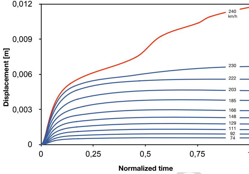
Figure 14: Diagrams time-displacement for various wind speeds v_0 .
