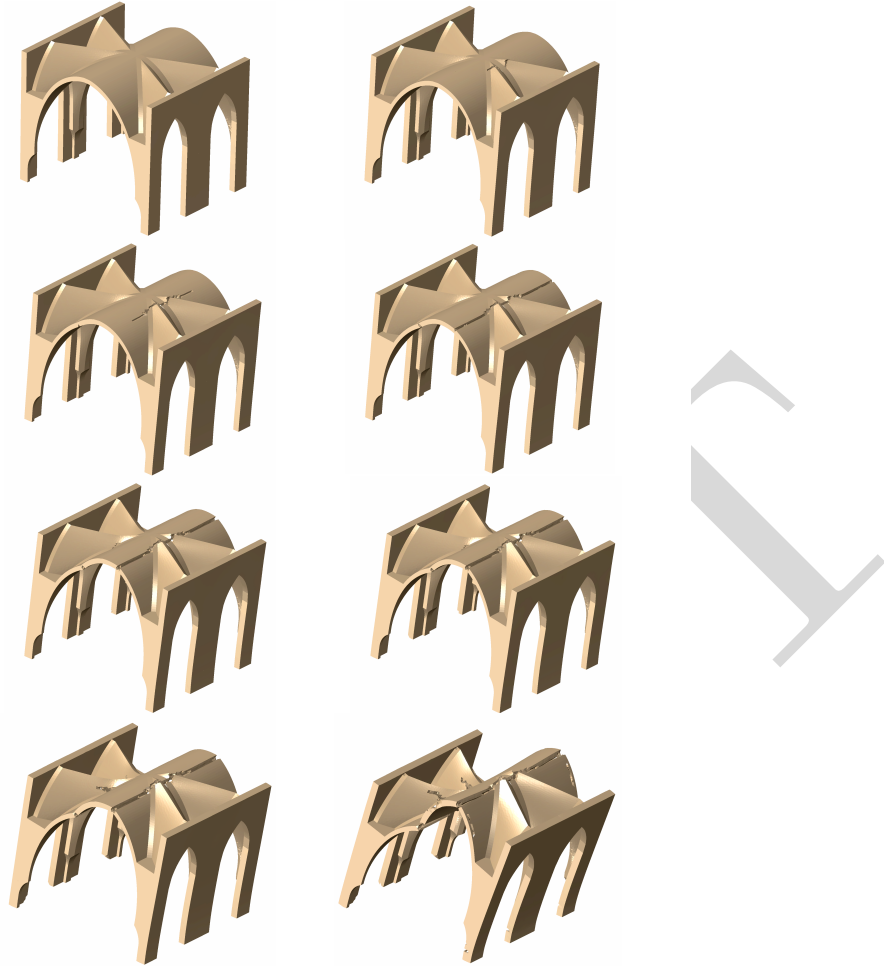
Figure 19: Progressive failure of the high sexpartite vault
