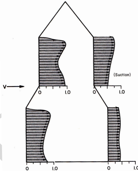
Figure 10: Distribution of C_D on a Gothic-Cathedral, according to [Mark, 1982].
