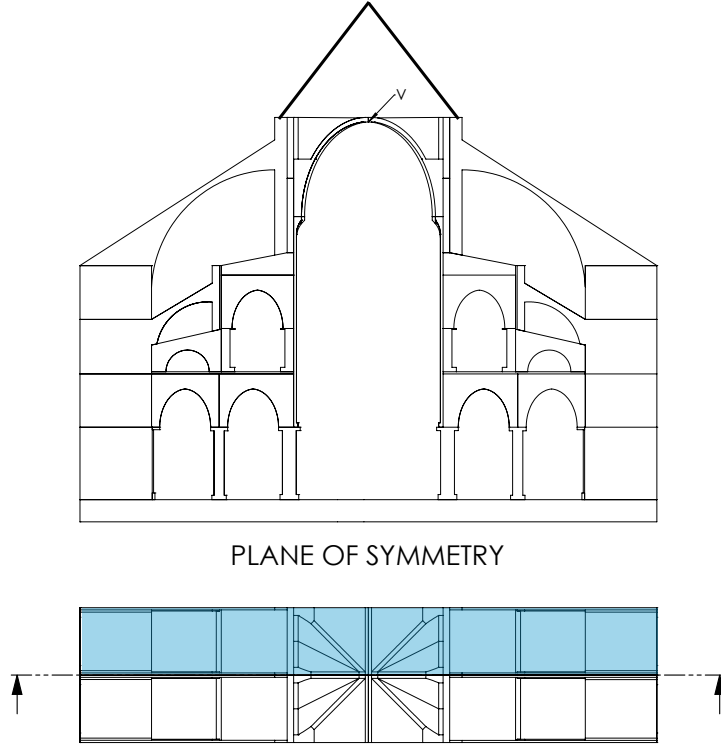
Figure 6: The part of the unit studied (highlighted in blue).
