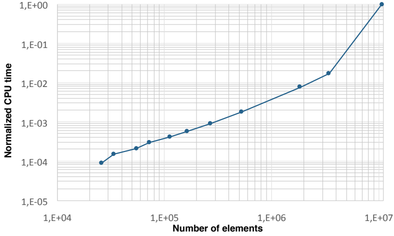
Figure 21: Normalized CPU times of the standard analyses versus the number of elements.
