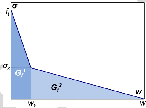
Figure 8: Traction-separation diagram and fracture energy.
