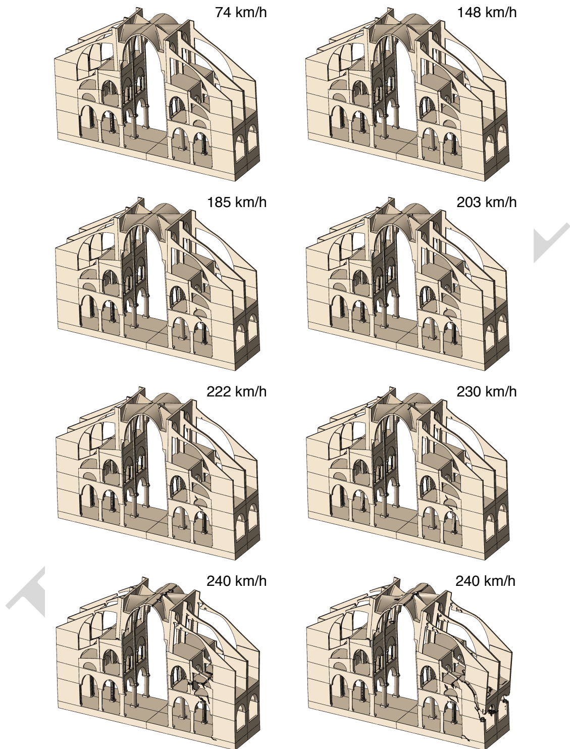
Figure 17: Progressive damage of the structure and formation of the collapse mechanism; the two last plots are for the same wind speed, but taken at two successive instants.
