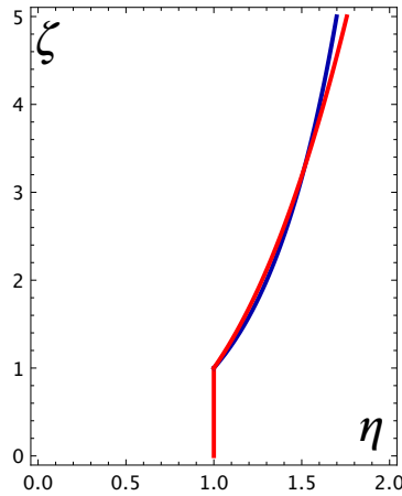
Figure 23: Comparison of the wind profiles given by power law (7), in red, and Eurocode 1, eq. (21), in blue.
