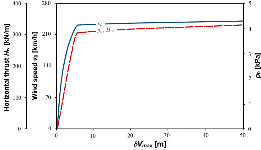
Figure 15: Wind speed v_0 , total horizontal wind thrust H_w and wind pressure p_0 versus the horizontal displacement of point V, \delta V_{max} .
