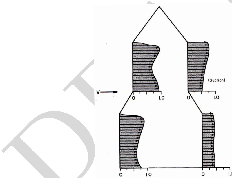
Figure 15: Distribution of C_D on a Gothic Cathedral, according to [Mark, 1982].
