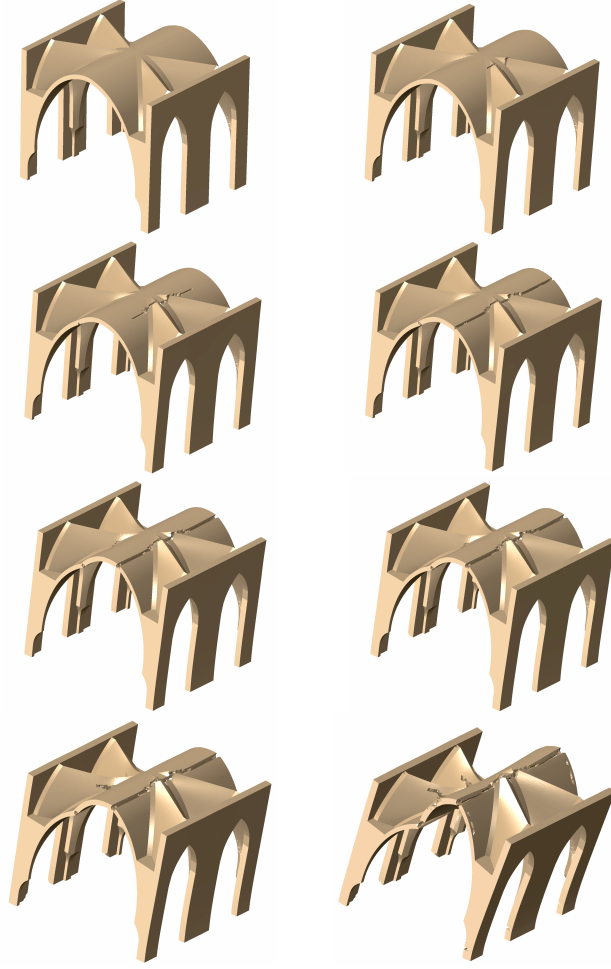
Figure 24: Progressive failure of the high sexpartite vault
