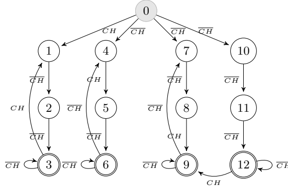
Fig. 6. Cyclic automaton for the crop CH with rt(CH) = 3 and \mathcal{H} - h = 4 .
