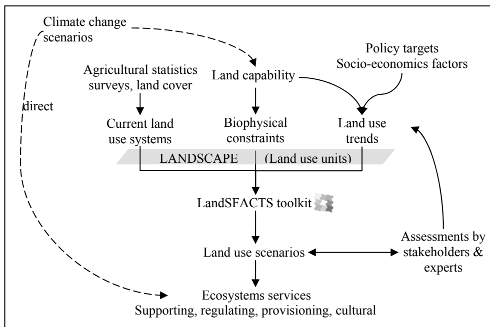
Figure 1: General framework
