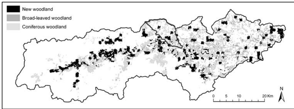
Figure 4: Scenarios of new woodland in the Dee catchment when aiming to enhance woodland network, while considering climate change.
