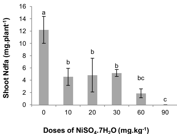
Fig. 7. Shoot nitrogen fixed from the air (Ndfa, \text{mg plant}^{-1} ) of lentils grown on soil contaminated with Ni. Means \pm confidence interval followed by different letters are significantly different at p < 0.05 (Tukey's multiple range test), ( n = 3 ).
