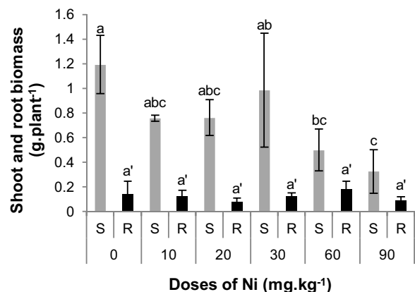
Fig. 1. Shoot (grey bars) and root (black bars) biomass ( g \text{ plant}^{-1} ) of lentils in relation to Ni additions ( mg \text{ kg}^{-1} ). Means \pm confidence interval followed by different letters are significantly different at p < 0.05 (Tukey's multiple range test), ( n = 3 ).
