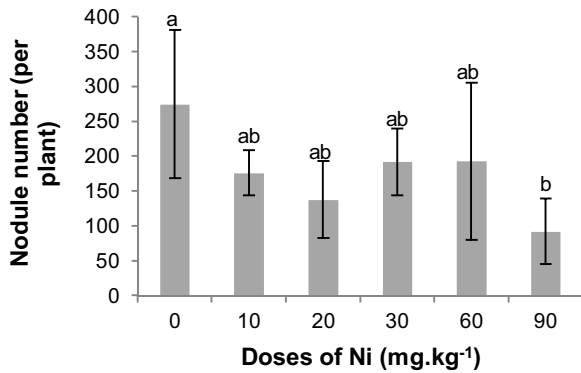
Fig. 6. Nodule number (per plant) of lentils in relation to Ni additions ( \text{mg kg}^{-1} ). Means \pm confidence interval followed by different letters are significantly different at p < 0.05 (Tukey's multiple range test), ( n = 3 ).
