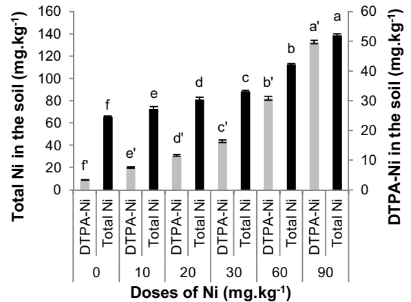
Fig. 8. Total nickel (total-Ni) (black bars) and DTPA-extractable nickel (DTPA-Ni) (grey bars) in the soil at the harvest ( \text{mg kg}^{-1} ). Means \pm confidence interval followed by different letters are significantly different at p < 0.05 (Tukey's multiple range test), ( n = 3 ).
