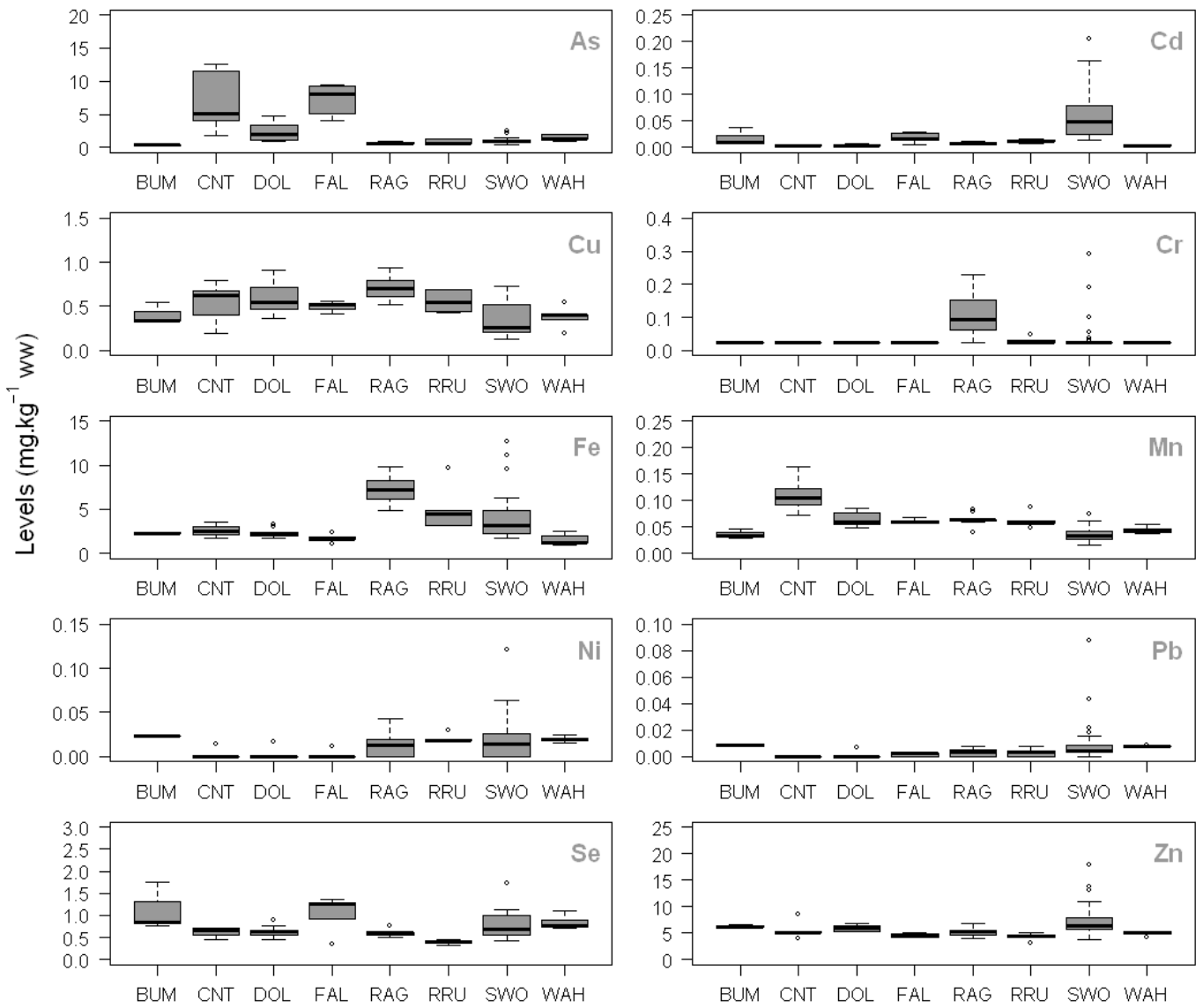
Fig. 3. Boxplots of trace element levels (ppm ww) in the muscle of eight oceanic pelagic fish species caught in the western-central Indian Ocean. BUM = Blue marlin, CNT = Rough triggerfish, DOL = Dolphinfish, FAL = Silky shark, RAG = Indian mackerel, RRU = Rainbow runner, SWO = Swordfish, WAH = Wahoo. Letters indicate significant differences between species.
