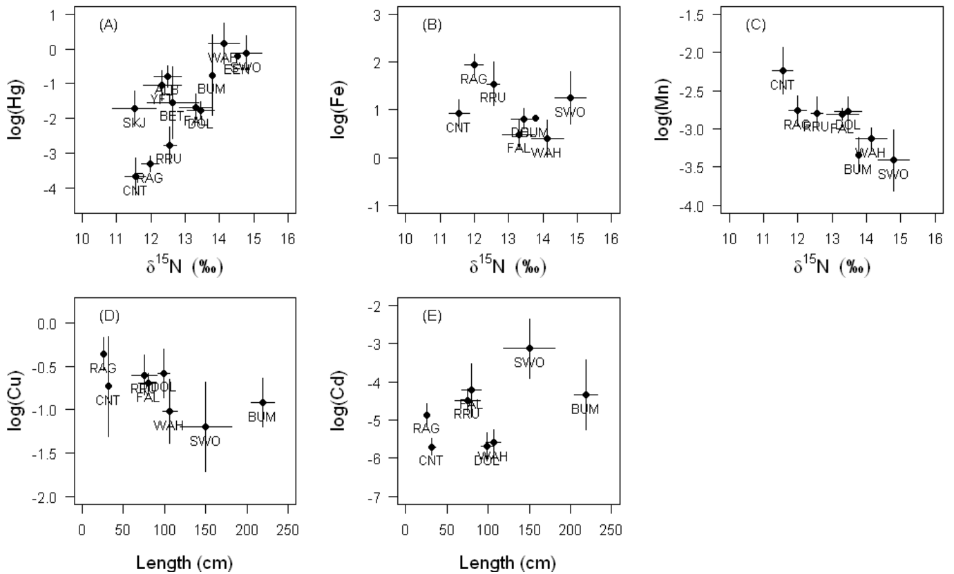
Fig. S2. Plots of significant relationships between (A) nitrogen stable isotope values ( \delta^{15}\text{N} ) and log-transformed Hg levels, (B) \delta^{15}\text{N} and log-transformed Fe levels, (C) \delta^{15}\text{N} and log-transformed Mn levels, (D) fish size (length, cm) and log-transformed Cu levels, and (E) fish size and log-transformed Cu levels, for oceanic pelagic fish species caught in the western-central Indian Ocean. ALB = Albacore tuna, BET = Bigeye tuna, BUM = Blue marlin, CNT = Rough triggerfish, DOL = Dolphinfish, EEN = Giant grouper, FAL = Silky shark, RAG = Indian mackerel, RRU = Rainbow runner, SKJ = Skipjack tuna, SWO = Swordfish, WAH = Wahoo, YFT = Yellowfin tuna.
