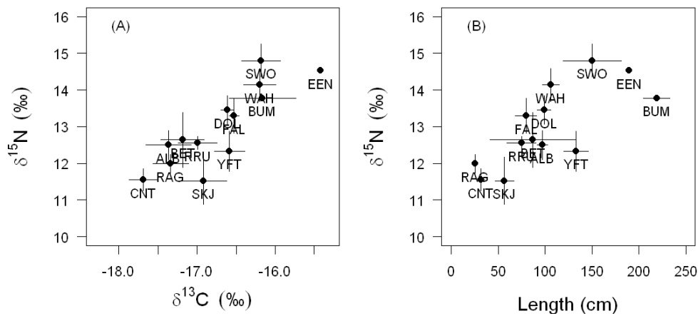
Fig. S1. Plots of mean \pm standard deviation of (A) carbon and nitrogen stable isotope ratios ( \delta^{13}\text{C} and \delta^{15}\text{N} ), and (B) fish size and \delta^{15}\text{N} for oceanic pelagic fish species caught in the western-central Indian Ocean. ALB = Albacore tuna, BET = Bigeye tuna, BUM = Blue marlin, CNT = Rough triggerfish, DOL = Dolphinfish, EEN = Giant grouper, FAL = Silky shark, RAG = Indian mackerel, RRU = Rainbow runner, SKJ = Skipjack tuna, SWO = Swordfish, WAH = Wahoo, YFT = Yellowfin tuna.
