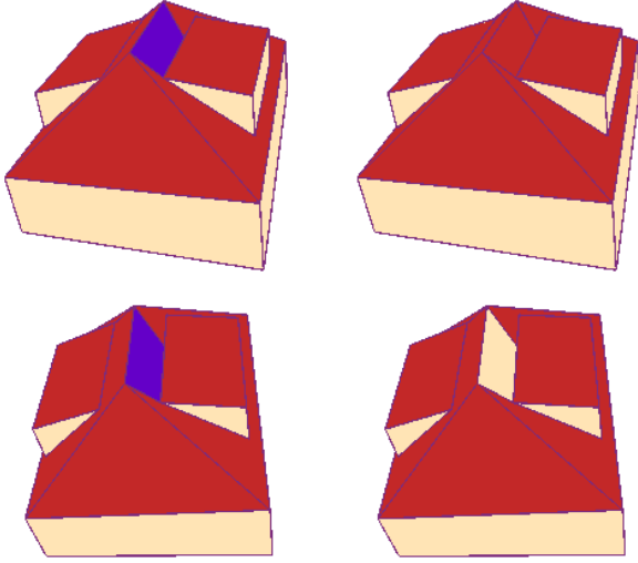
Figure 6: Example of a semantic difference spotted by the comparison algorithm. The top view is the EBM-LCC that comes from the OBJ file, the bottom view is the EBM-LCC that comes from the CityGML file. On the left this is a view that color semantic differences in purple so that the user can spot it easily. On the right this is the normal view with regular semantic associated color.
