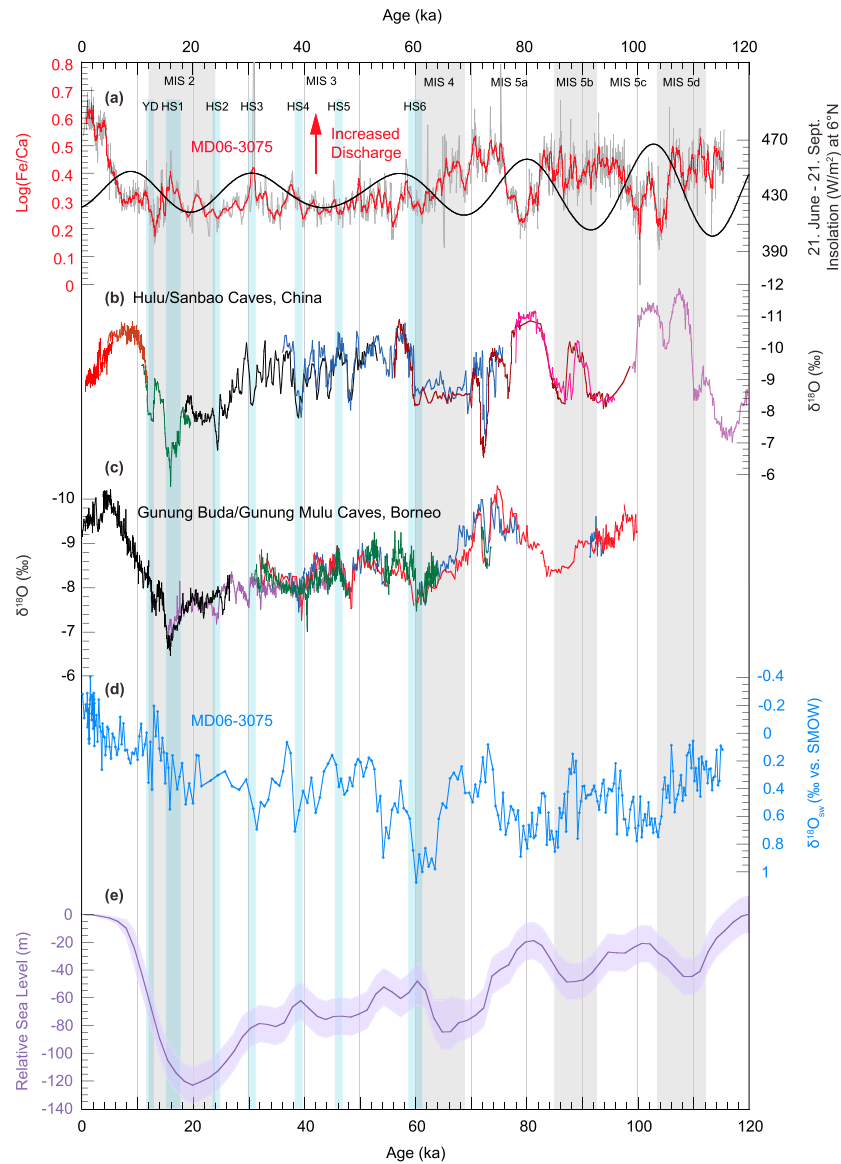
Figure 6. (a) XRF records of log(Fe/Ca) from Core MD06-3075 superimposed with mean boreal summer (21 June to 21 September) insolation at 6°N. (b) Composite speleothem \delta^{18}\text{O} records from Hulu and Sanbao caves in China [Wang et al. , 2001, 2008]. (c) Composite speleothem \delta^{18}\text{O} records from Gunung Mulu and Gunung Buda Caves in Borneo [Partin et al. , 2007; Carolin et al. , 2013]. (d) Estimated ice-volume corrected \delta^{18}\text{O}_{\text{sw}} from \delta^{18}\text{O} measurements on G. ruber and \text{U}^{\text{K}}_{37} -derived SSTs in Core MD06-3075. (e) Relative sea level change based upon Waelbroeck et al. [2002]. Grey vertical bars indicate major marine isotope stages, blue vertical bars indicate HS1–HS6 and the YD.
