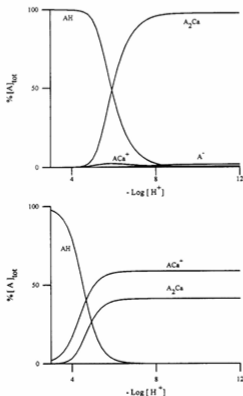
Figure 4. Formation curves of calcium cezomycin complexes under various acidic conditions: (a, top) [A] tot = 2 × 10 -4 mol L -1 , [Ca 2+ ] = 10 -4 mol L -1 ; (b, bottom) [A] tot = 10 -4 mol L -1 , [Ca 2+ ] = 1.7 × 10 -2 mol L -1 . Solvent = methanol; T = (25.0 ± 0.1) °C; I = 0.1 M.
