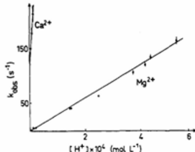
Figure 5. Dissociation of the cezomycin calcium and magnesium A_2M complexes: variations of the pseudo-first order rate constants with proton concentrations. Solvent = methanol; T = (25.0 \pm 0.1)^\circ\text{C} ; I = 0.1\text{ M} .
