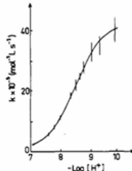
Figure 6. Formation of the neutral magnesium cezomycin A_2Mg complex: variations of the second-order rate constants with proton concentrations. Solvent = methanol; T = (25.0 \pm 0.1)^\circ\text{C} ; I = 0.1\text{ M} .
