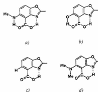
Figure 7. Hydrogen bonds in monoprotonated species of calcimycin and closely related ionophores: (a) calcimycin; (b) X 14885A; (c) cezomycin; (d) N -methylcalcimycin.
