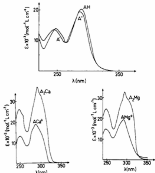
Figure 3. Calculated electronic spectra for various protolytic species of the free antibiotic cezomycin and its calcium and magnesium complexes: (a, top) deprotonated and monoprotonated free cezomycin species; (b, bottom left) calcium cezomycin complexes; (c, bottom right) magnesium cezomycin complex es. Solvent = methanol; T = (25.0 ± 0.1) °C; I = 0.1 M.
