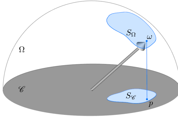
Figure 2: The irradiance of a hemispherical domain is the fraction of the unit disk covered by its projection.
