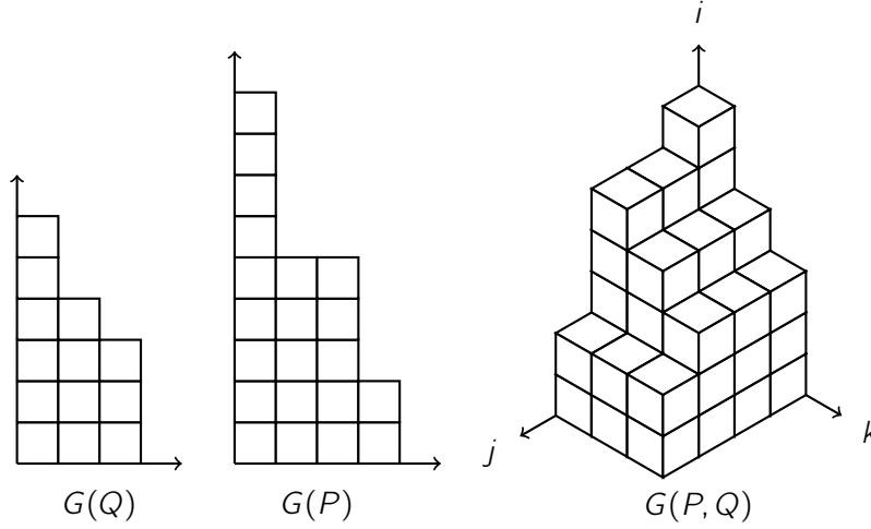
Figure 2: Merge of two Greene diagrams.
