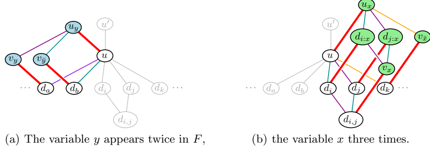
Fig. 1. General structure of the graph G_F , with the two possible examples of gadgets associated to a variable. Red edges correspond to the cut M_y on (a) and M_x on (b).
