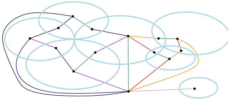
Fig. 3. A (non-simple) non-separating set of Jordan curves and its region graph.
