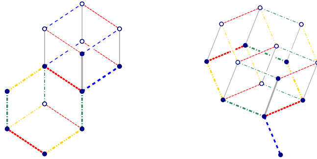
Fig. 4. Two ULDs obtained from the same partial cube (thick edges) by fixing a different vertex.
