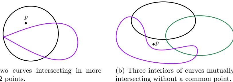
Fig. 2. Illustration of Observation 10. In both cases p is a point proving that the arrangement is not non-separating.
