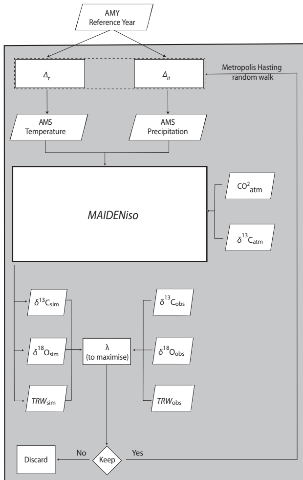
Figure 1. MAIDENiso’s inversion flowchart. For each year simulated, two \Delta modify the AMY: one for temperature ( \delta_{Tt} ) and one for precipitation ( \delta_{\pi t} ). The resulting AMS is passed to MAIDENiso, along with atmospheric \text{CO}_2 concentrations and atmospheric \delta^{13}\text{C} to simulate tree growth parameters. Simulated tree growth is compared to observations, through the metric \lambda , which has to be maximized (Eq. 1). The Metropolis–Hastings algorithm iteratively modifies the value of \delta_T and \delta_\pi so that it converges towards stable states (Eq. 2).
