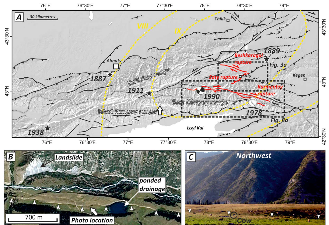
Figure 2. (a) Shaded-relief SRTM topography of the Zailisky And Kungey Tien Shan, showing the major active faults (in black, from our own mapping). Earthquake ruptures from the 1911 earthquake are shown in white, and those potentially associated with the 1889 earthquake are shown in red. The Chon Kemin and Chon Aksu ruptures of the 1911 earthquake are simplified from Arrowsmith et al. [2015]. The potential 1889 ruptures are from our own work, following initial observations by Tibaldi et al. [1997] and Crosby et al. [2007]. The isoseismals of the 1889 earthquake are from Arrowsmith et al. [2015] digitized from maps drawn by Djanuzakov et al. [2003]. Black stars represent the epicenters of historical earthquakes [ Kulikova and Krüger , 2015]. The white arrow shows the location of Figures 2b and 2c. (b) Google Earth image of part of the Chon Aksu rupture. The south facing rupture is visible as a white stripe (marked by white arrows). It has uplifted the valley floor and blocked a small north flowing stream to form a pond. A landslide from 1911 is visible in the top left of the image. (c) Field photograph looking NW at the 1911 ruptures. White arrows mark the base of scarp. Scale provided by cows.
