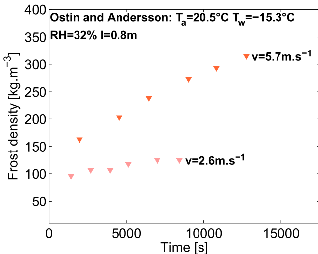
Fig. 20 – Impact of environmental parameters on frost density: air velocity.
