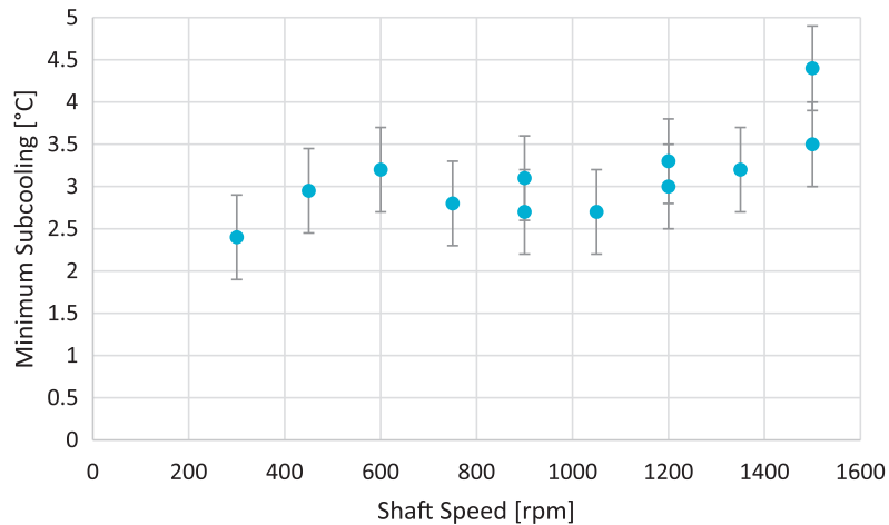
Fig. 11. Evolution of the minimum subcooling with pump shaft speed.
