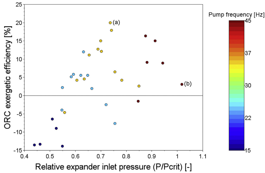
Fig. 13. ORC exergetic efficiency function of relative pressure for constant HTF temperature of 95 °C.
