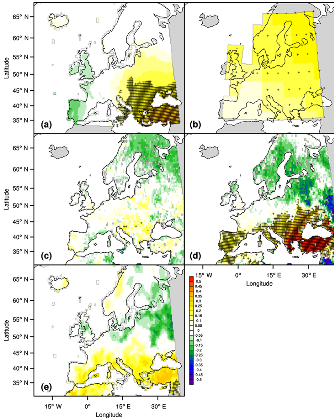
Figure 8. Spatial correlation maps for the March–April temperature reconstruction and precipitation signal ( PC_1 ) obtained from the tree-ring dataset during the period 1800–2002 over Europe. Maps demonstrate spatial field correlations between our temperature reconstruction and (a) gridded spring temperature reconstruction for Europe (Xoplaki et al., 2005), (b) gridded summer temperature reconstruction for Europe (Luterbacher et al., 2016), (c) Old World Drought Atlas (OWDA; Cook et al., 2015). Panels (d) and (e) show spatial correlations between PC_1 and OWDA (Cook et al., 2015) and gridded European summer precipitation reconstruction (Pauling et al., 2006), respectively. The + sign represents significant correlation coefficients ( p < 0.05 ).
