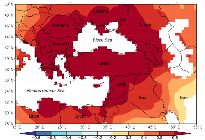
Figure 7. Spatial correlation map for the March–April temperature reconstruction. Spatial field correlation map showing statistical relationship between the temperature reconstruction and the gridded temperature field at 0.5^\circ intervals (CRU TS3.23; Jones and Harris, 2008) during the period 1930–2002 over the Mediterranean region. For each grid, calculated correlation coefficient from 0.20 to 0.60 is significant ( p < 0.05 ).
