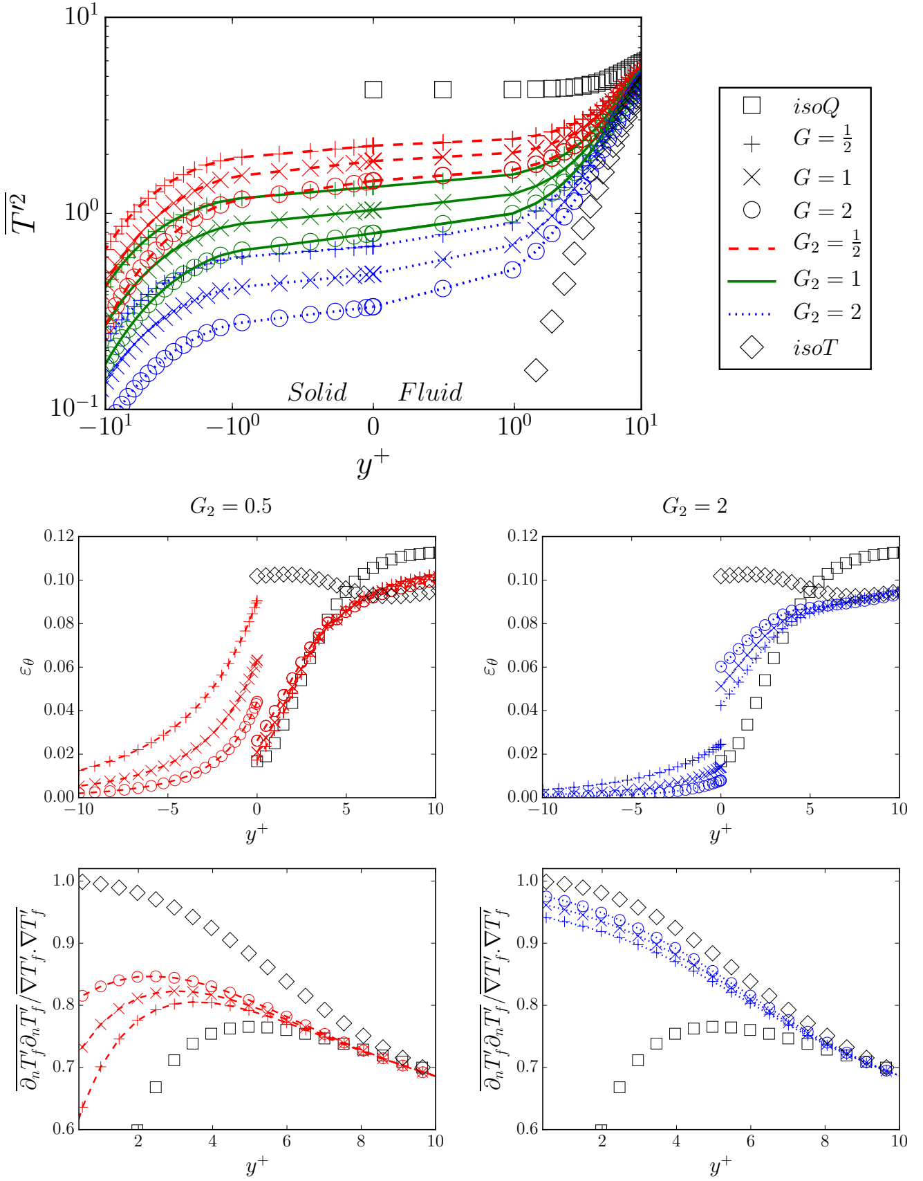
Figure 1: Top: temperature variance \overline{T'^2} . Middle: dissipation rate \varepsilon_\theta . Bottom: relative contribution of the wall-normal part in the temperature gradient \frac{\partial_n T'_f \partial_n T'_f}{\nabla T'_f \cdot \nabla T'_f} . Left: CHT_{*0} . Right: CHT_{*2} .
