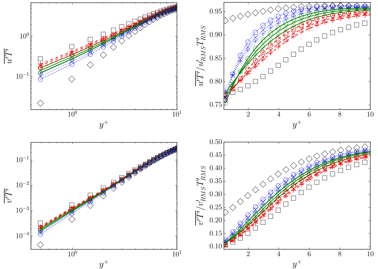
Figure 2: Top: streamwise heat flux. Bottom: wall-normal heat flux. Left: turbulent heat flux. Right: one-point correlation coefficient associated with the turbulent heat flux. Lines and symbols as in figure 1.
