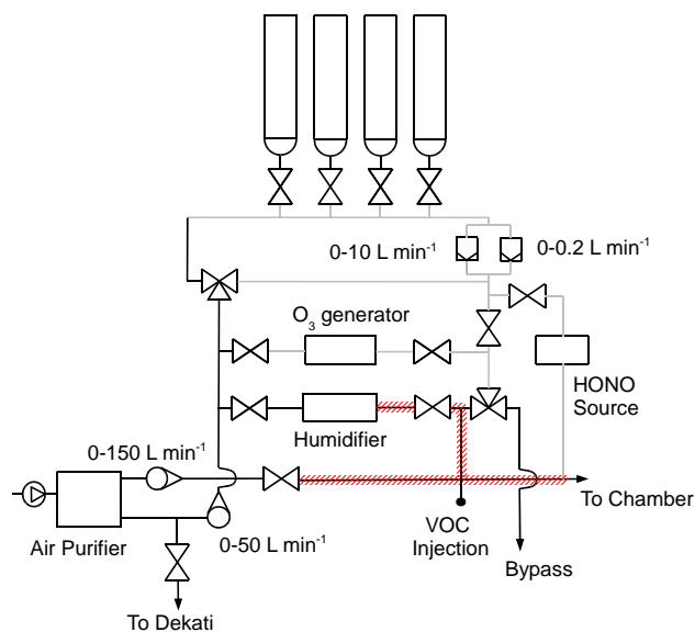
Fig. 2. Schematic (not to scale) of the primary component injection system of the mobile chamber. Pure air may be injected directly into the chamber through the main injection line, an insulated 12 mm (outer diameter) stainless steel tube which can be heated up to a maximum of 150 °C (red hatching, “To Chamber”). All or part of the pure air stream may be diverted through different sections of the primary injection system using a series of two- and three-way valves.
