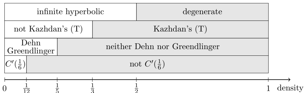
Figure 2: Phase transitions for properties of random presentations in the density model.
