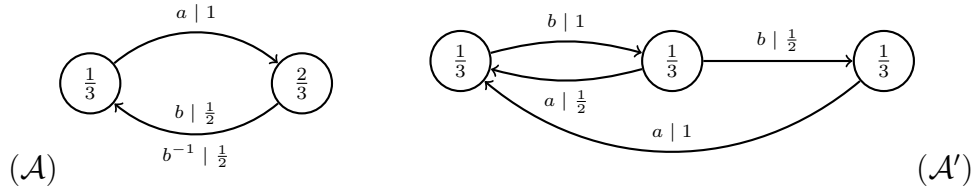
Figure 3: Markovian automata \mathcal{A} and \mathcal{A}' . Transitions are labeled by a letter and a probability, and each state is decorated with the corresponding initial probability.
