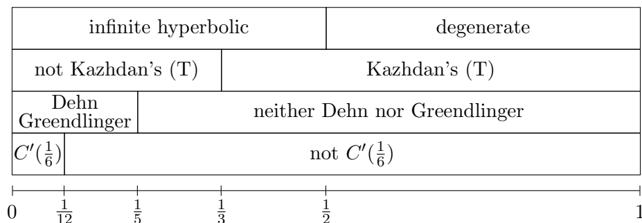
Figure 1: Phase transitions for properties of random presentations in the density model.
