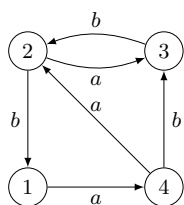
Figure 2: The Stallings graph of H = \langle aab, ab\bar{a}b, abbb \rangle . The reduced word u = aab\bar{a}b is in H as it is accepted by \Gamma(H) : it labels a path starting from 1 and ending at 1, with edges being used backward when reading a negative letter. Since every vertex has valency at least 2, this graph is cyclically reduced.
