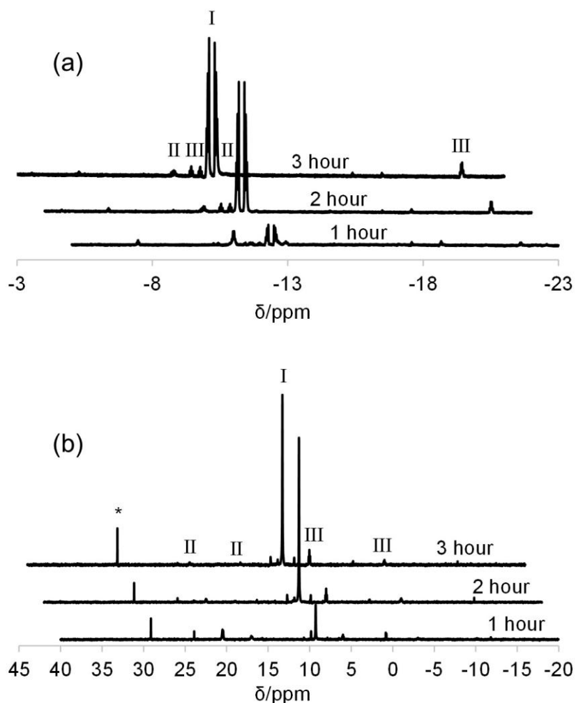
Figure 3. Monitoring by ^1\text{H} NMR in the hydride region (a) and ^{31}\text{P}\{^1\text{H}\} (b) of the reaction between [\text{IrCl}(\text{COD})]_2 , \text{PPh}_3 (4 equiv) and excess \text{NaOMe} in boiling i\text{PrOH} . The spectra were taken from dried aliquots redissolved in \text{CDCl}_3 . The starred resonance is assigned to the \text{Ph}_3\text{PO} impurity.
