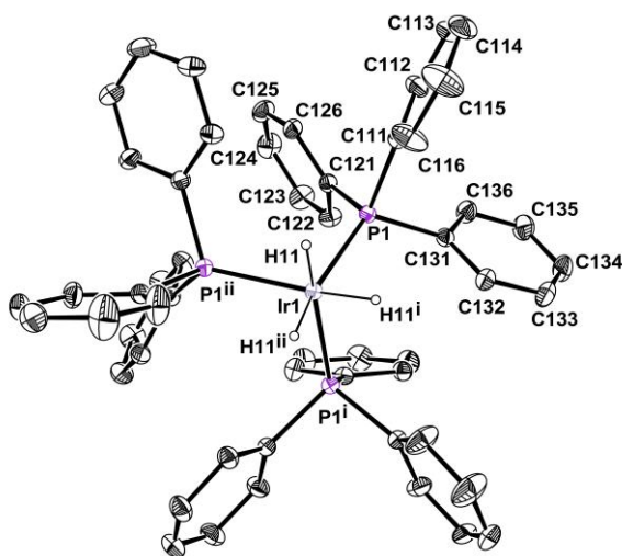
Figure 5. ORTEP view of fac -[IrH 3 (PPh 3 ) 3 ]. Relevant structural parameters: Ir-P, 2.3296(5); Ir-H, 1.39(5) Å; P-Ir-P i , 103.021(16); H-Ir-P, 89.7(19); H-Ir-P i , 84(2); H-Ir-P ii , 164(2)°. Symmetry codes: (i) 1-y, x-y, z; (ii) -x+y, 1-x, z.
