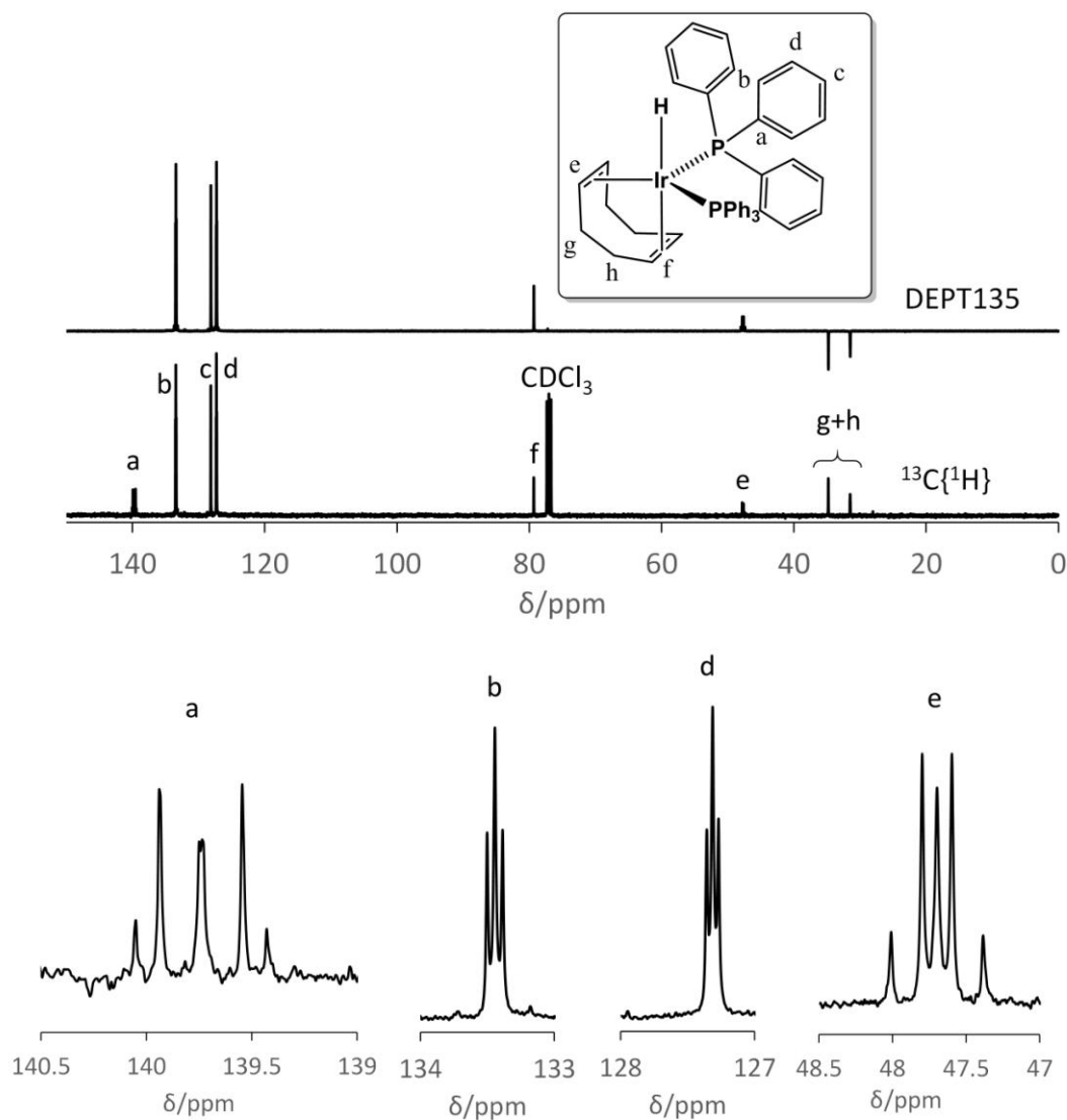
Figure 2. ^{13}\text{C}\{^1\text{H}\} and DEPT135 NMR spectra of [\text{IrH}(\text{COD})(\text{PPh}_3)_2] , with expanded excerpts for the C atoms exhibiting virtual coupling to the two P atoms.
