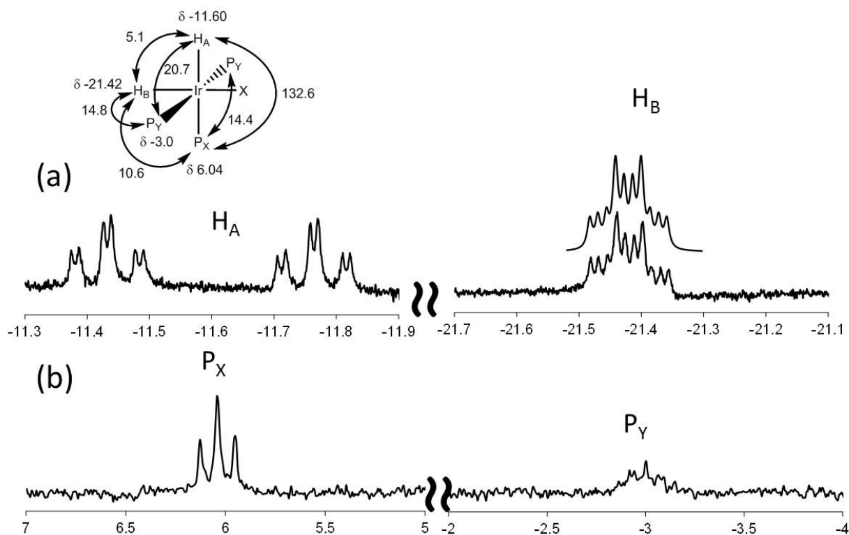
Figure 4. ^1\text{H} (a) and ^{31}\text{P}\{^1\text{H}\} (b) NMR properties of the minor product III resulting from the reaction between [\text{IrCl}(\text{COD})]_2 , \text{PPh}_4 (4 equiv) and excess \text{NaOMe} in boiling i\text{PrOH} . The upper trace for the \text{H}_\text{B} resonance is the simulated spectrum using the parameters indicated in the molecular diagram (in Hz units).
